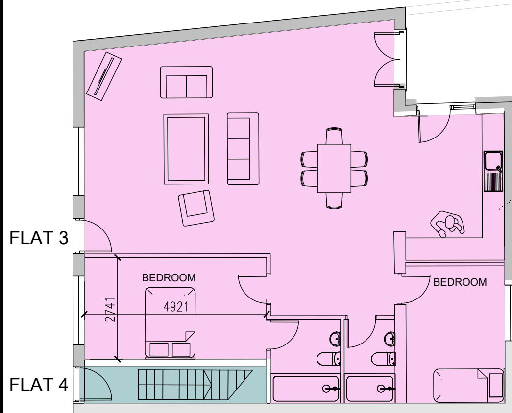
GROUND FLOOR PLAN - FLAT 2
