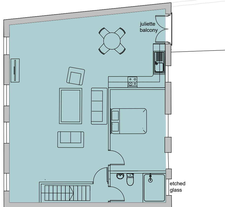
FIRST FLOOR PLAN - FLAT 3
