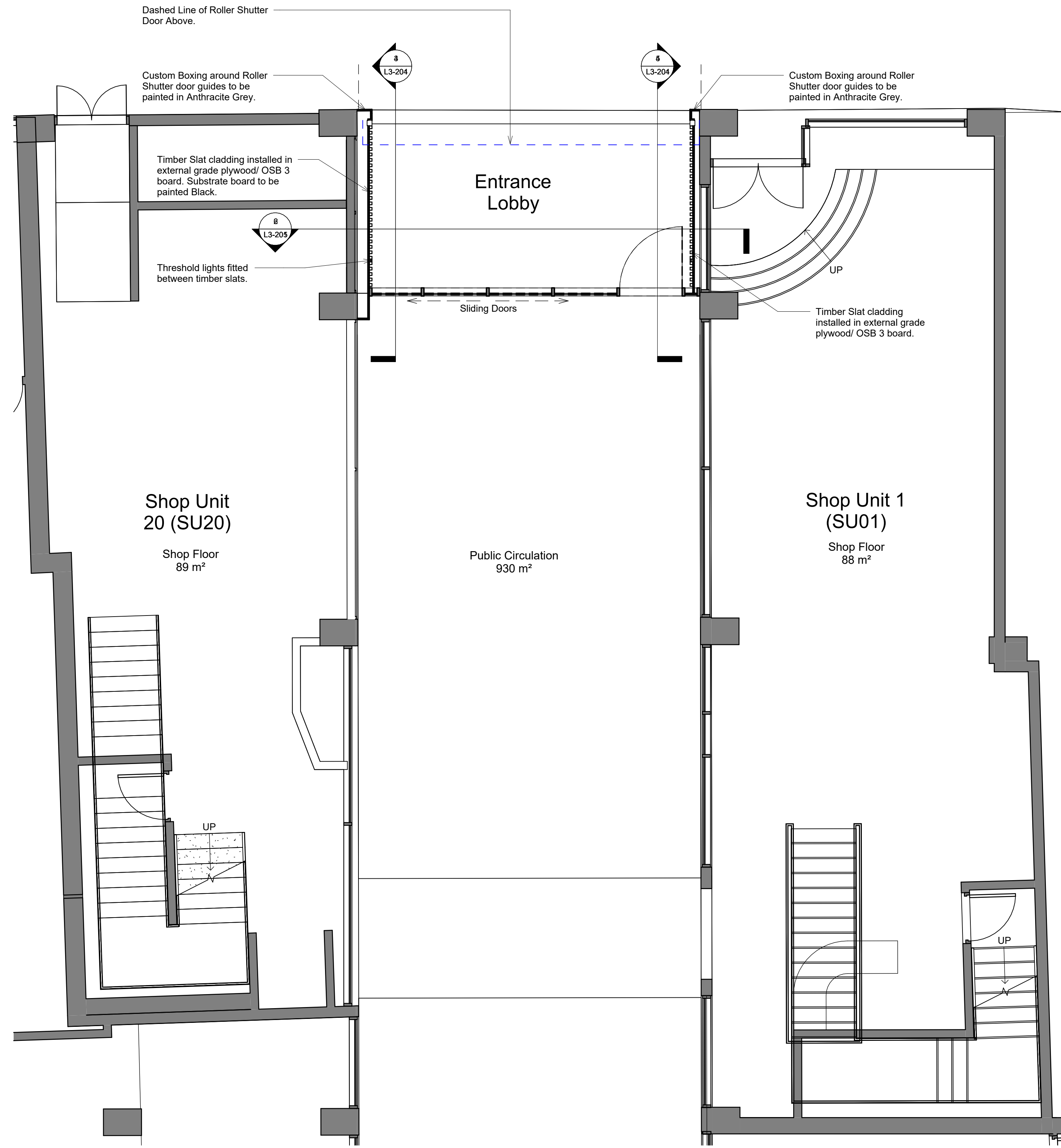
2 Entrance Lobby Plan (Proposed) 1 : 50
