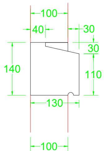
Brickwork Sill
