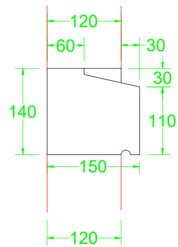
Render Sill
