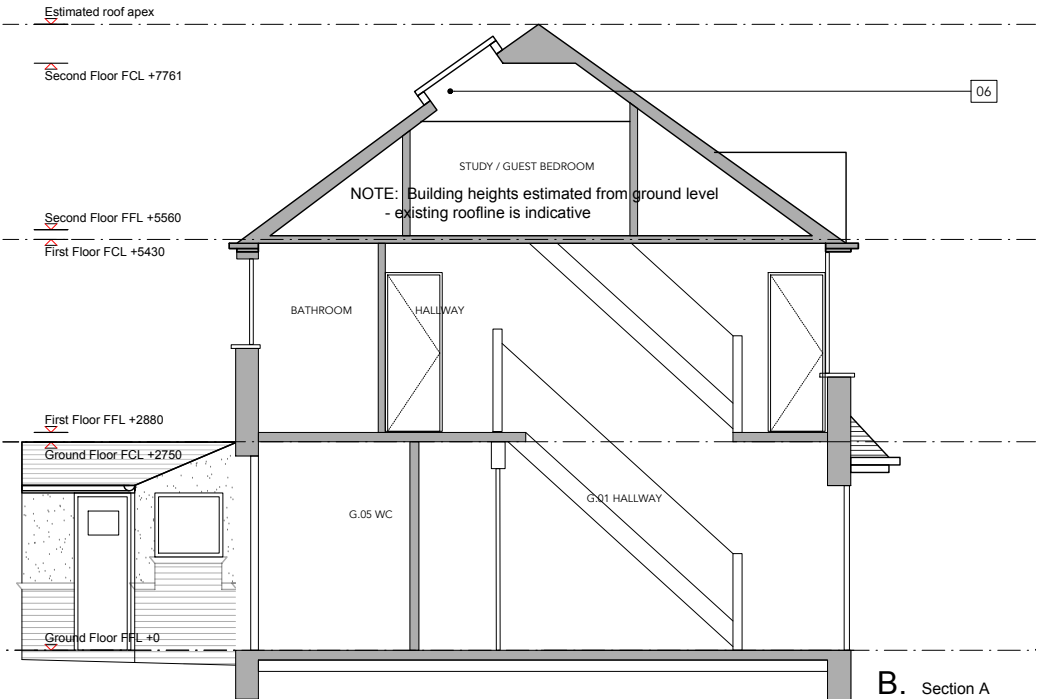
B. Section A
