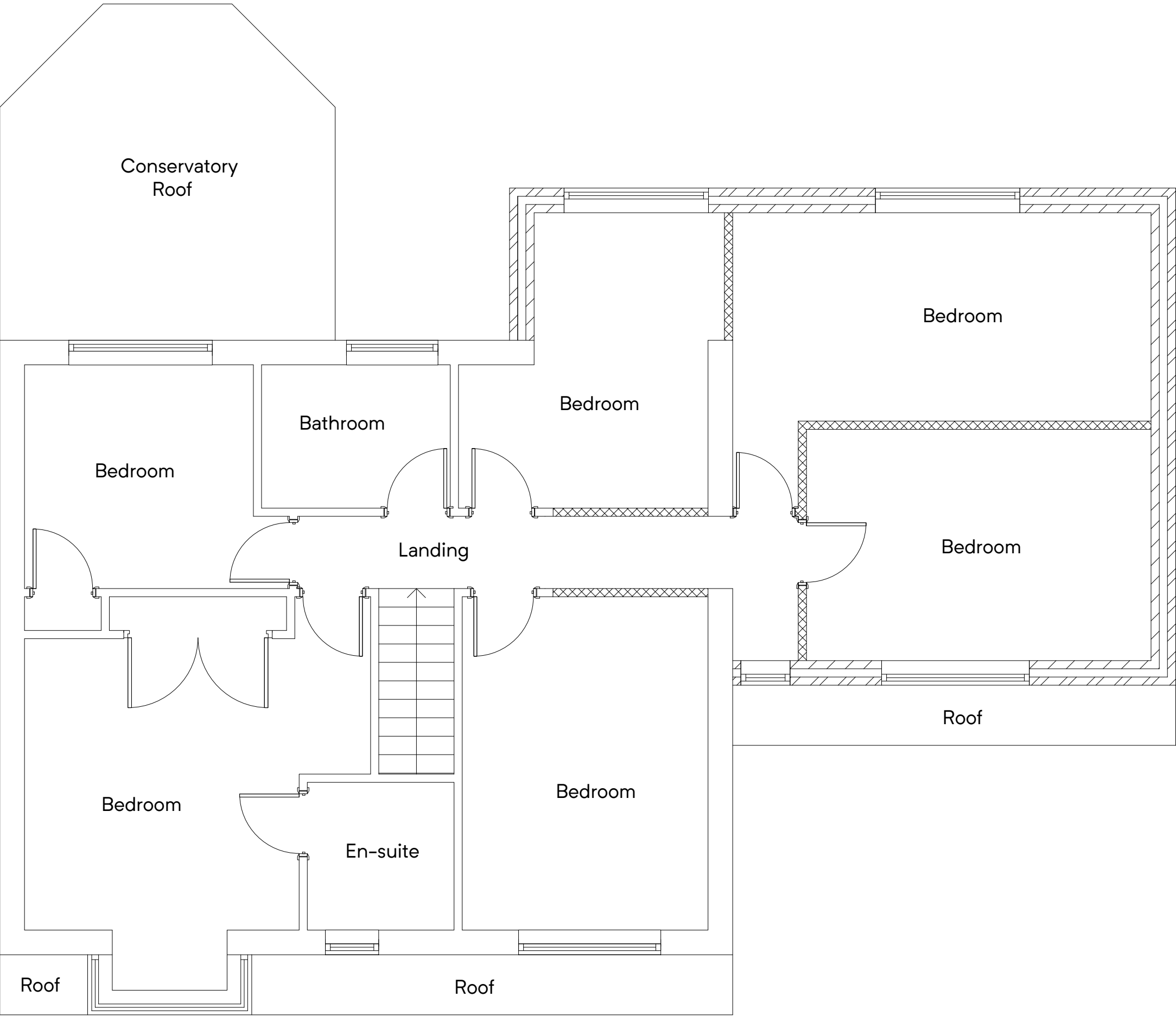
FIRST FLOOR PLAN (PROPOSED)
