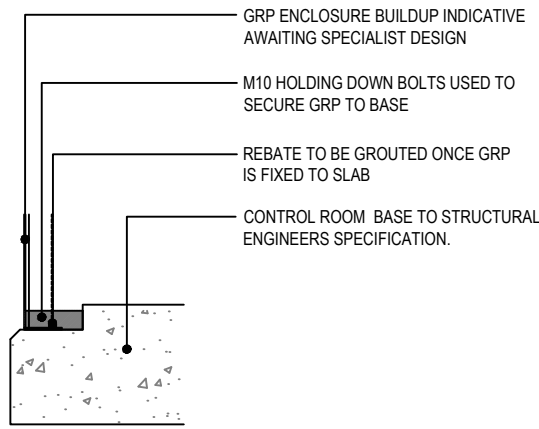
BASE REBATE DETAIL SCALE 1:20
