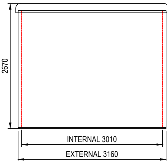
RIGHT HAND SIDE ELEVATION SCALE 1:50
