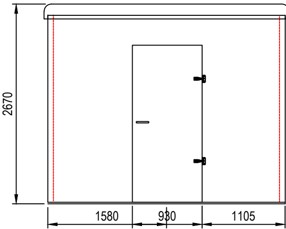
LEFT HAND SIDE ELEVATION SCALE 1:50
