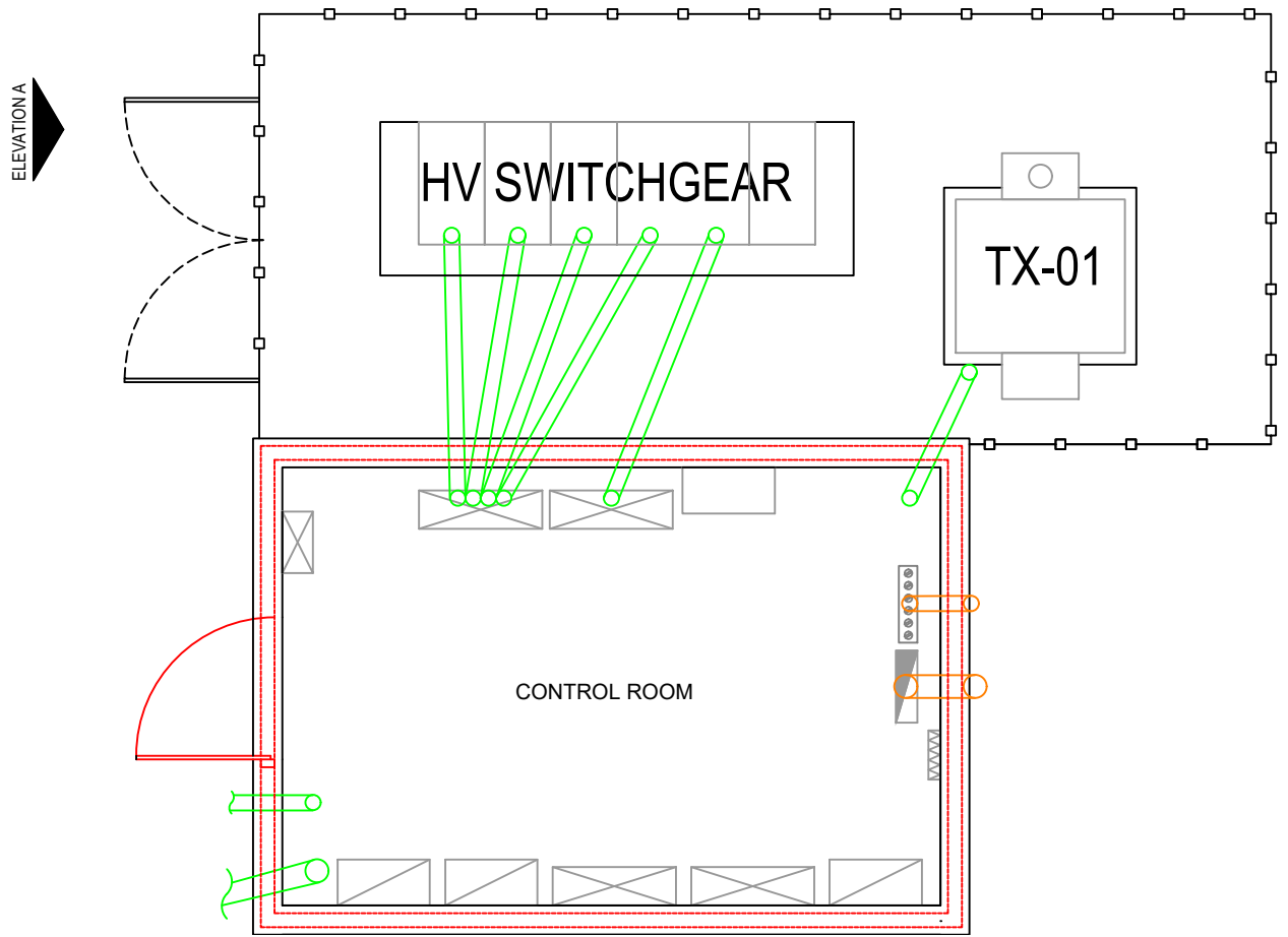
SUBSTATION GENERAL ARRANGEMENT SCALE 1:50
