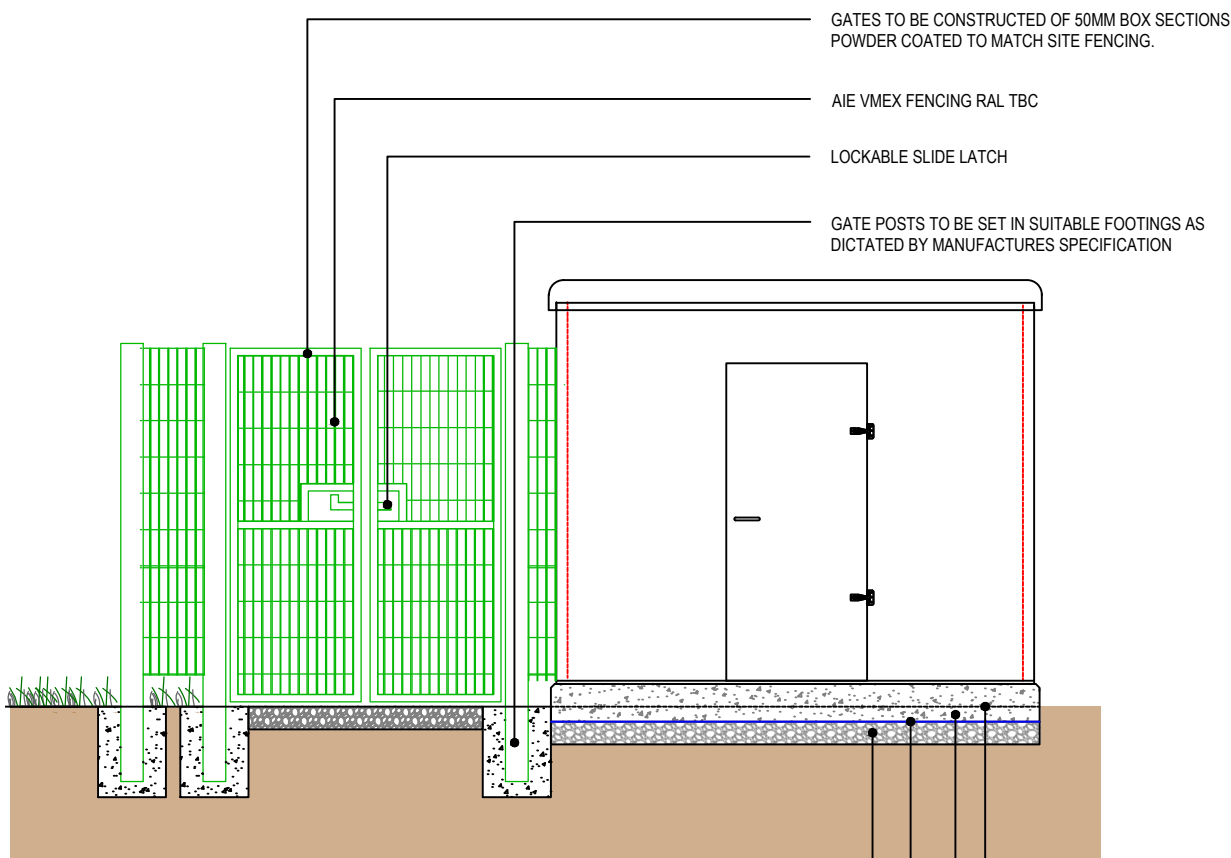
ELEVATION A - PROPOSED GATE AND SUBSTATION ARRANGEMENT ELEVATION SCALE 1:50
