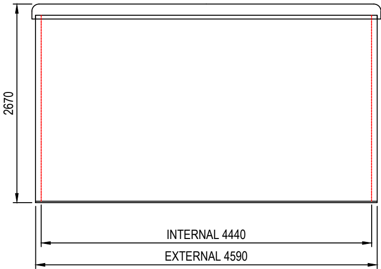
FRONT ELEVATION SCALE 1:50
