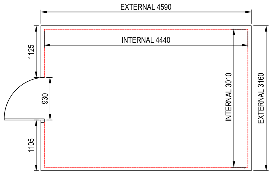
CONTROL ROOM GRP PLAN VIEW SCALE 1:50
