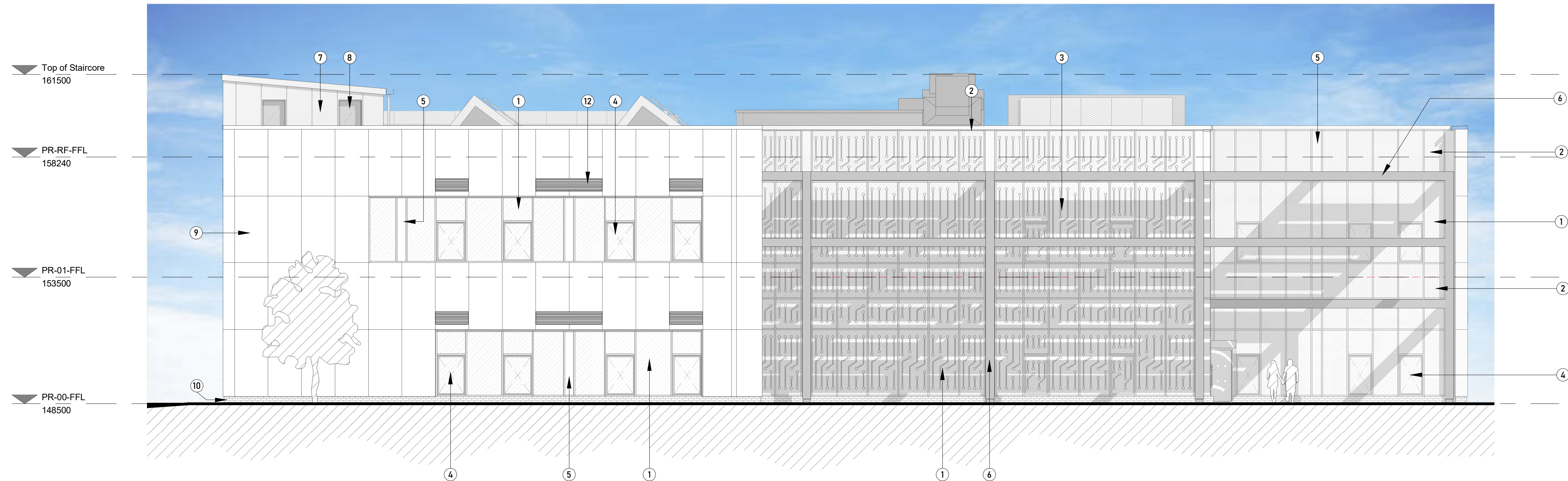
South Elevation 1 : 100
