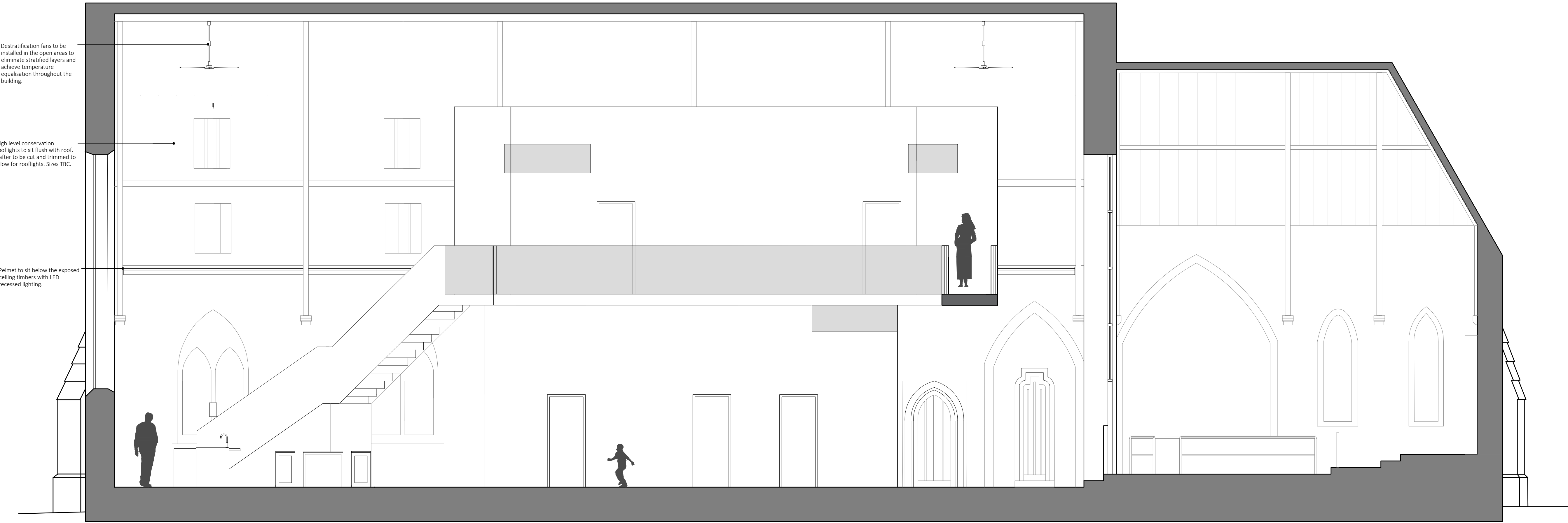
Section C-C
