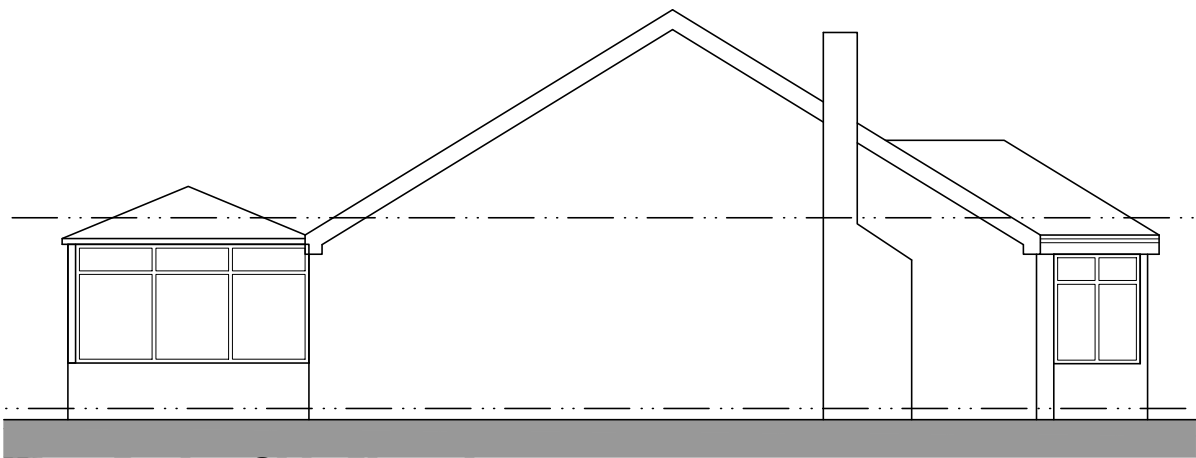
West Facing Side Elevation
