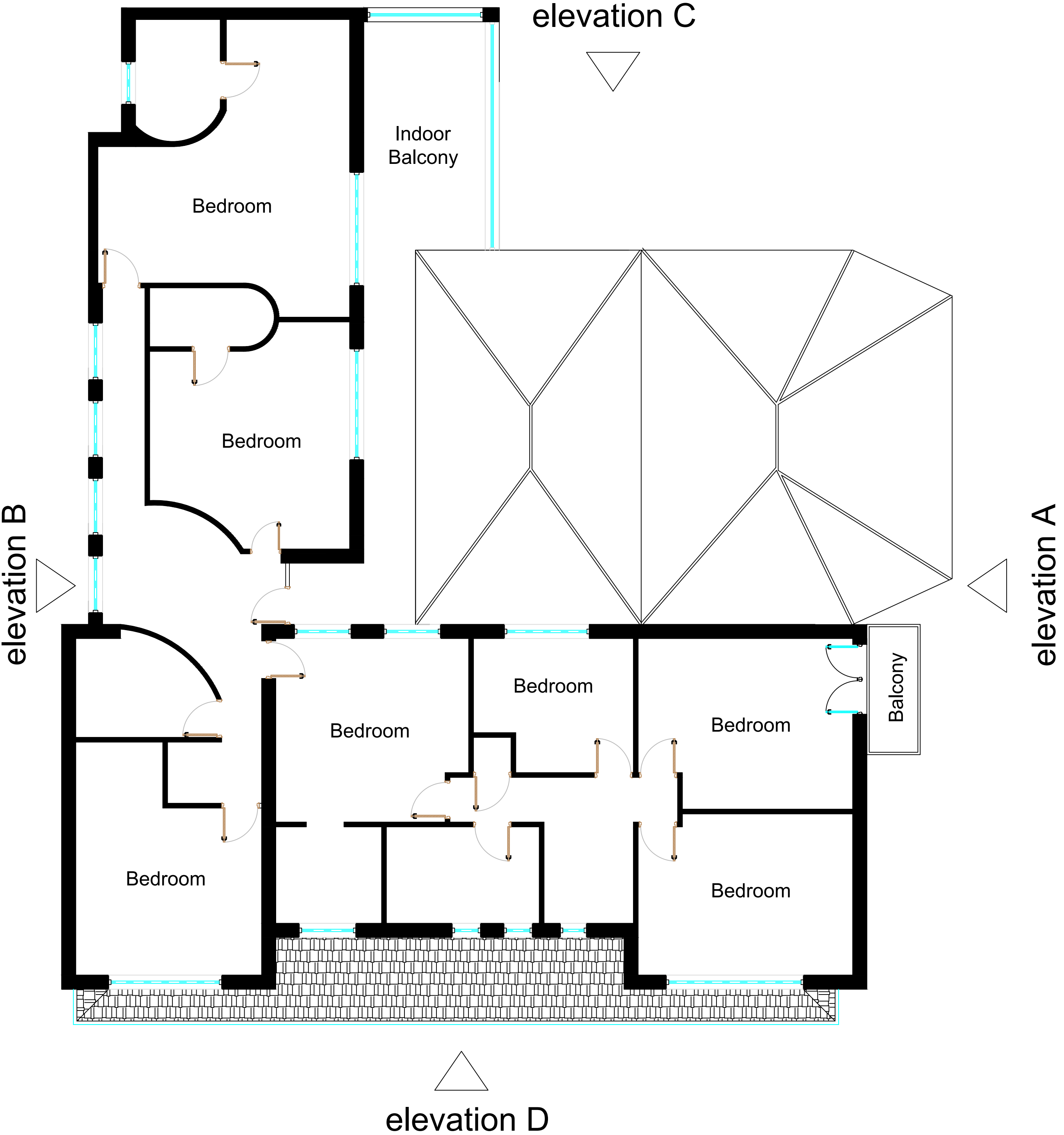
EXISTING FIRST FLOOR PLAN 1:50 @ A1
