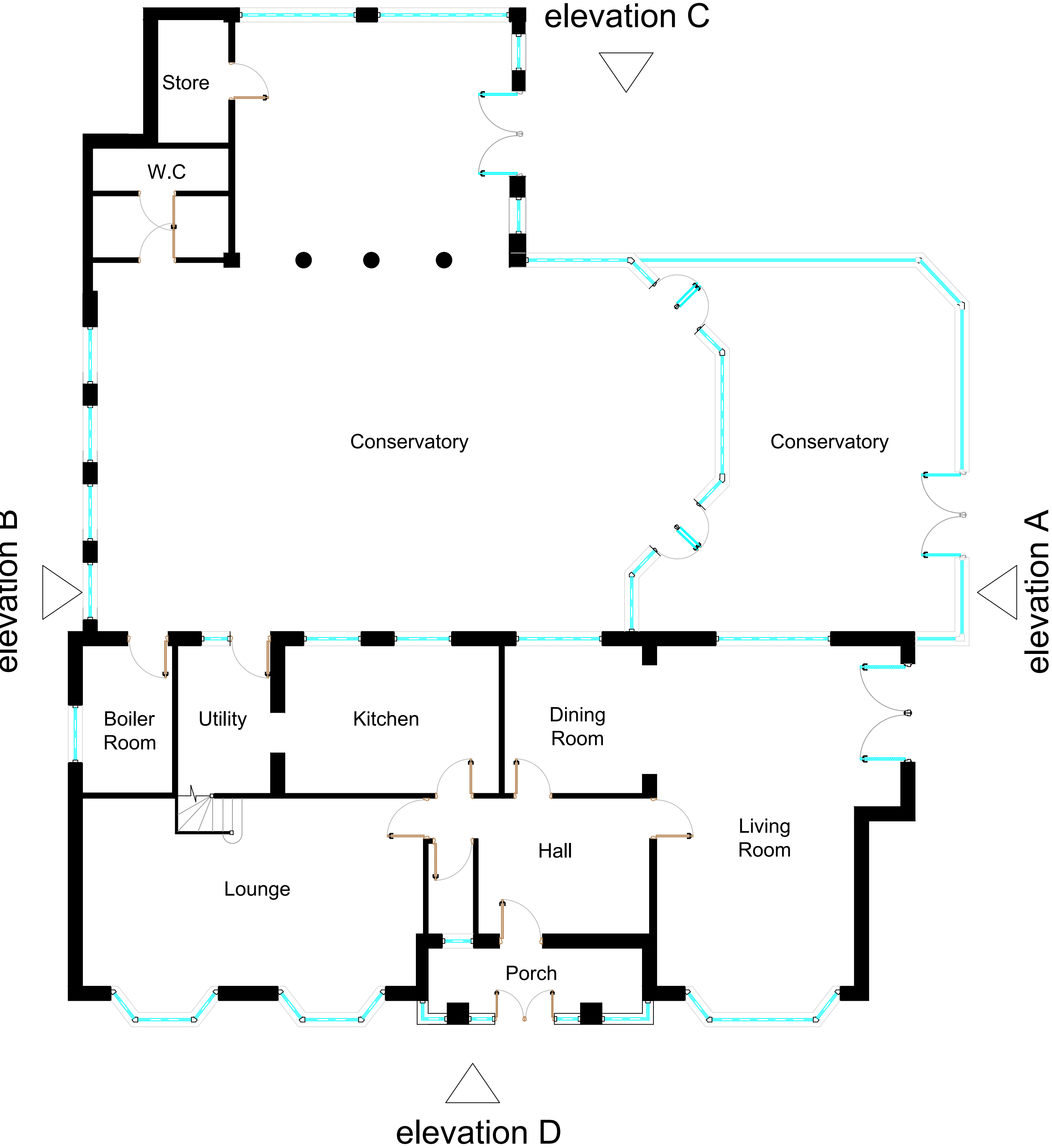
EXISTING GROUND FLOOR PLAN 1:50 @ A1
