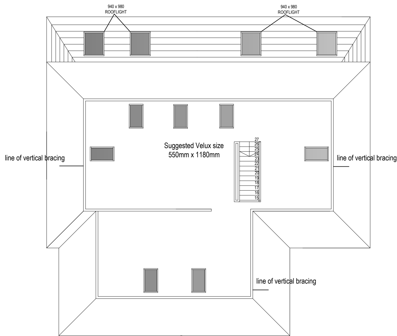
ATTIC PLAN
