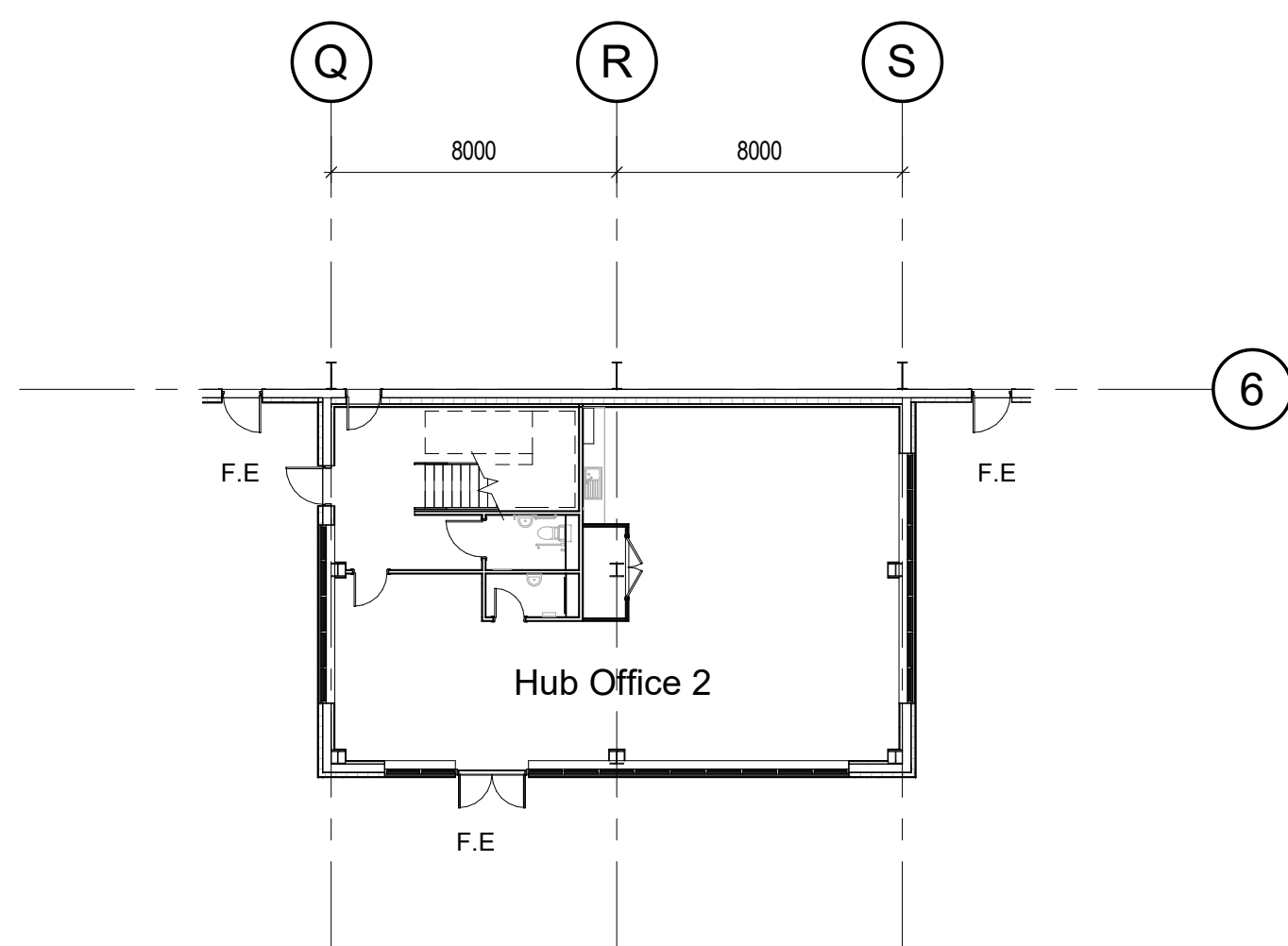
3 Ground Floor Hub Office 2 Scale @ 1 : 200
