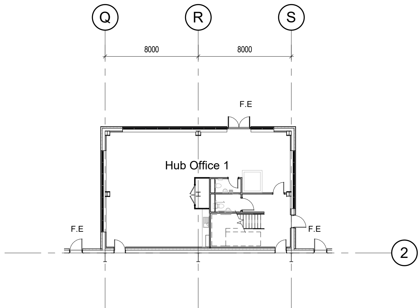
2 Ground Floor Hub Office 1 Scale @ 1 : 200
