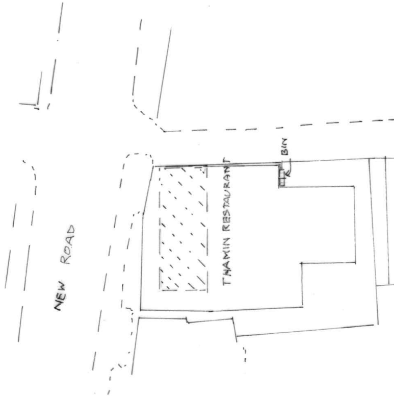
SITE PLAN (PROPOSED) SCALE 1:500
