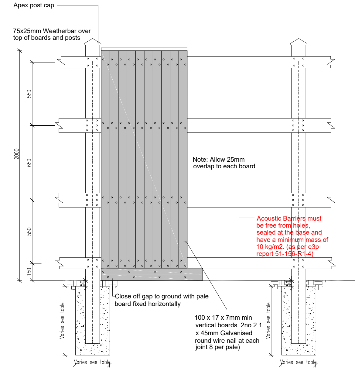
Acoustic Fence 2000-2800mm
