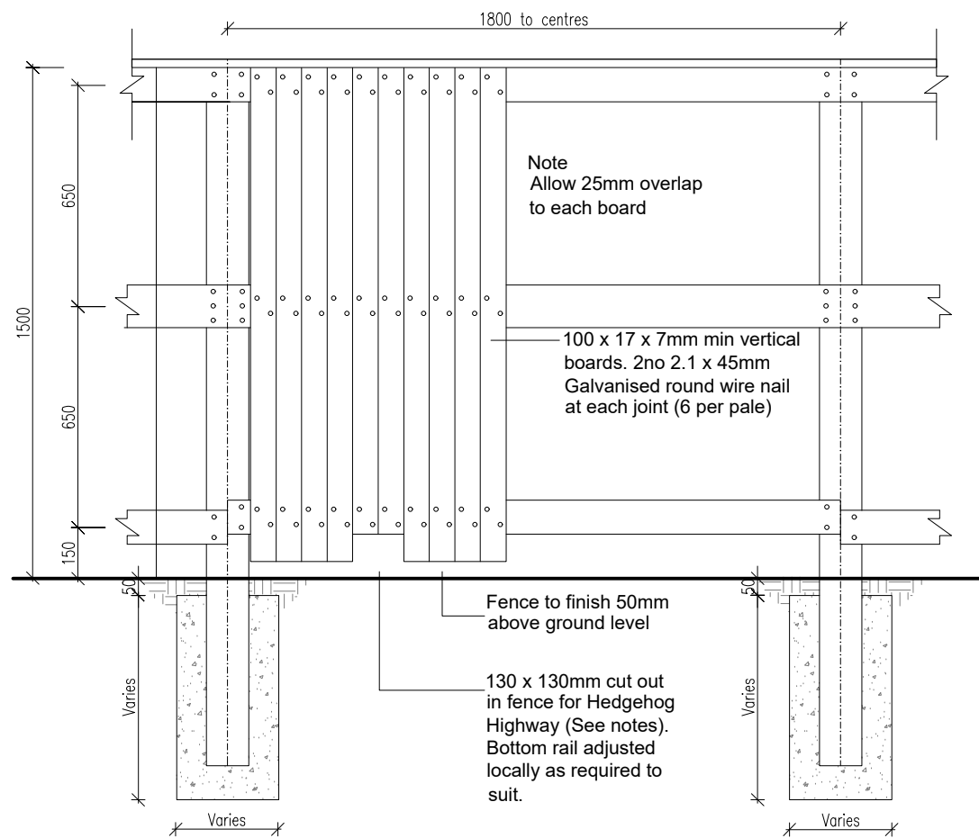
1.5m Fence
