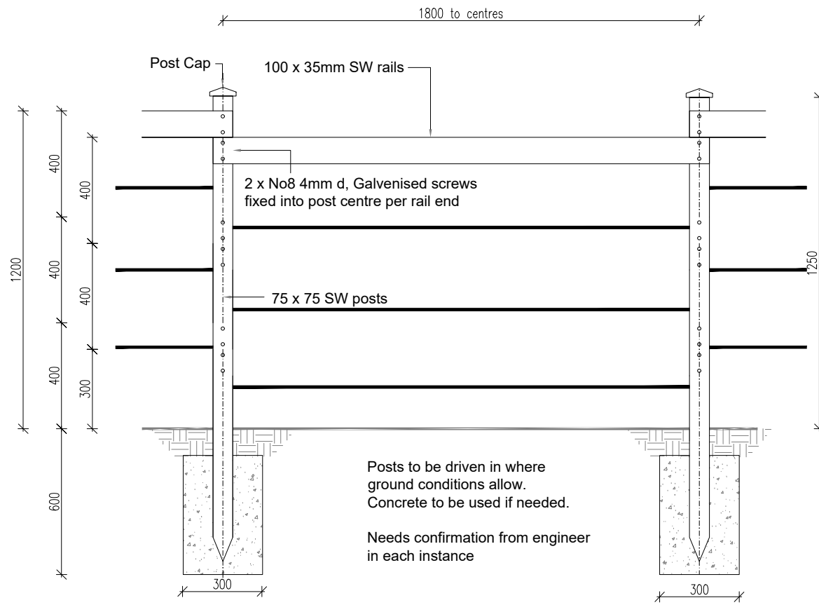
1200mm Post and Wire Fence
