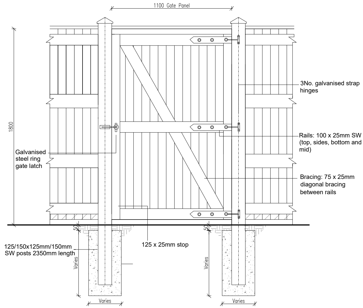
1.8m Gate
