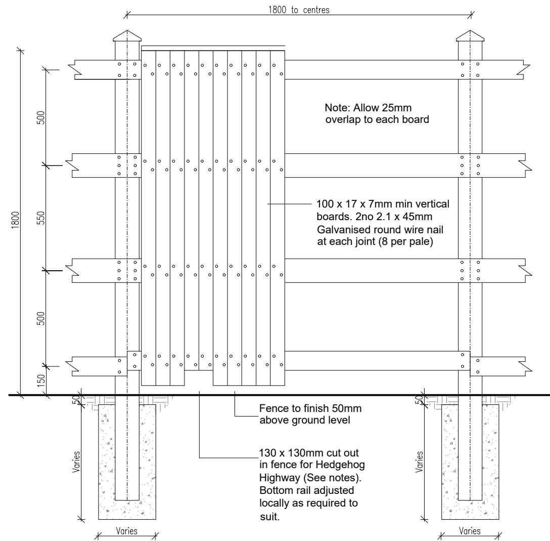
1.8m Fence
