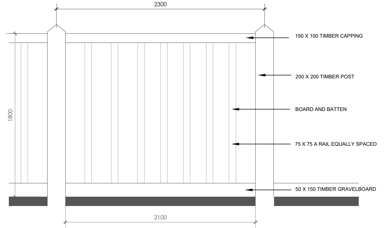
1800mm Screen Boundary Fence
