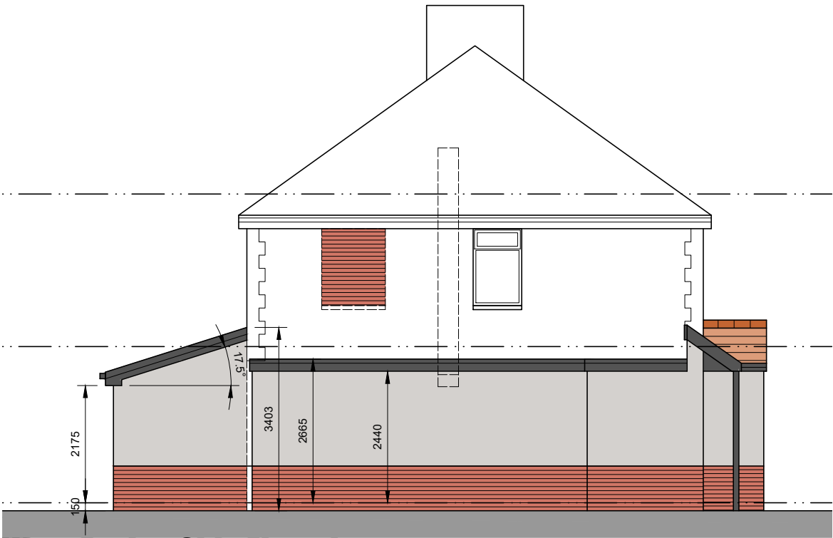
West Facing Side Elevation
