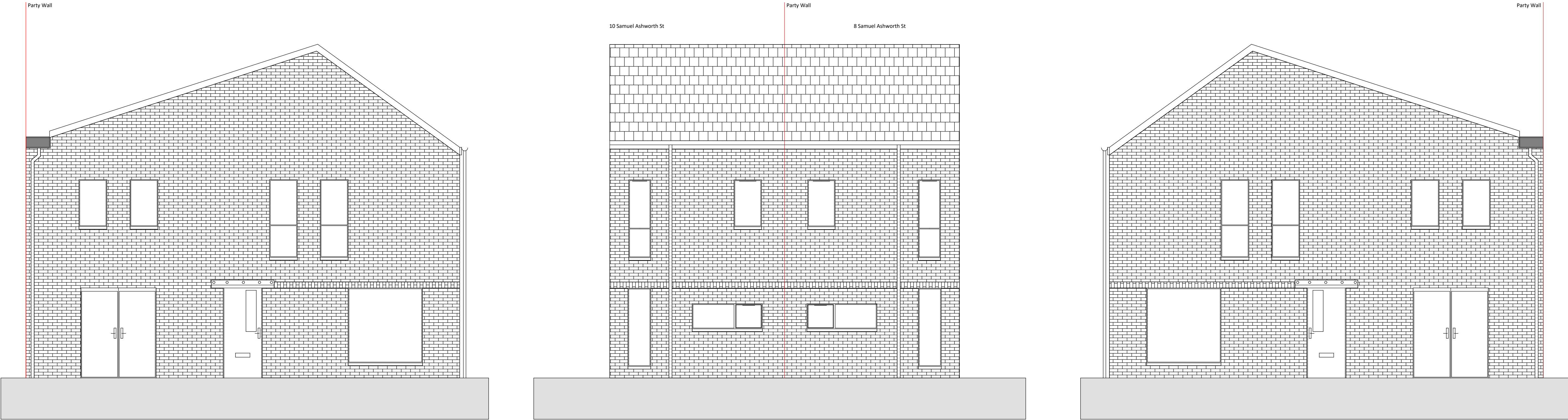
8/10 Samuel Ashworth St Existing Elevations 1 : 50
