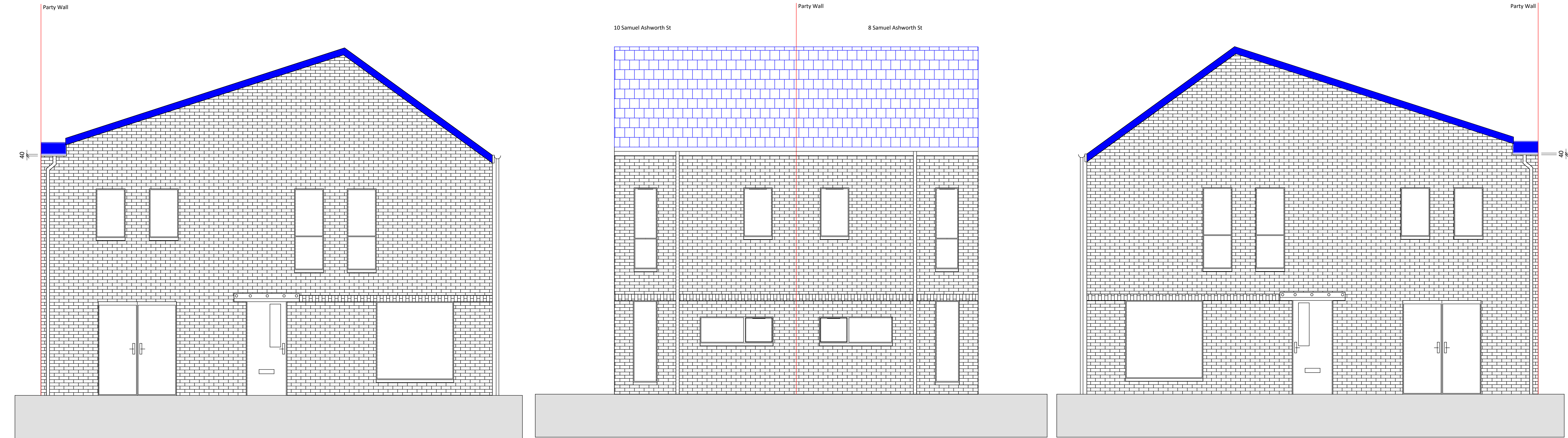
8/10 Samuel Ashworth St Proposed Elevations 1 : 50
