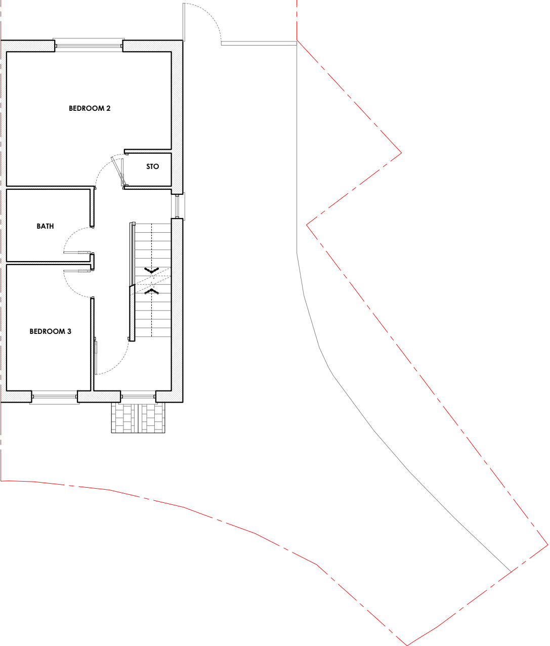
EXISTING FIRST FLOOR PLAN 1:100 @ A3
