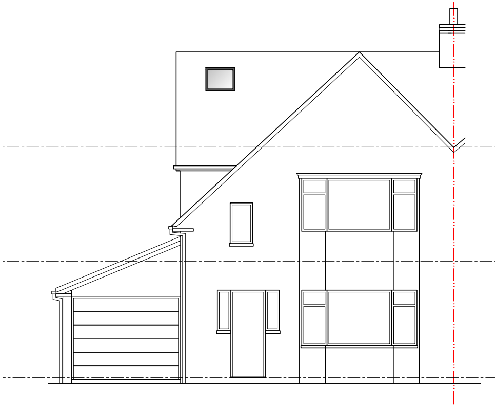
North Facing Front Elevation
