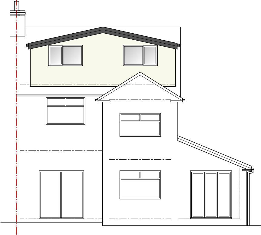
South Facing Rear Elevation
