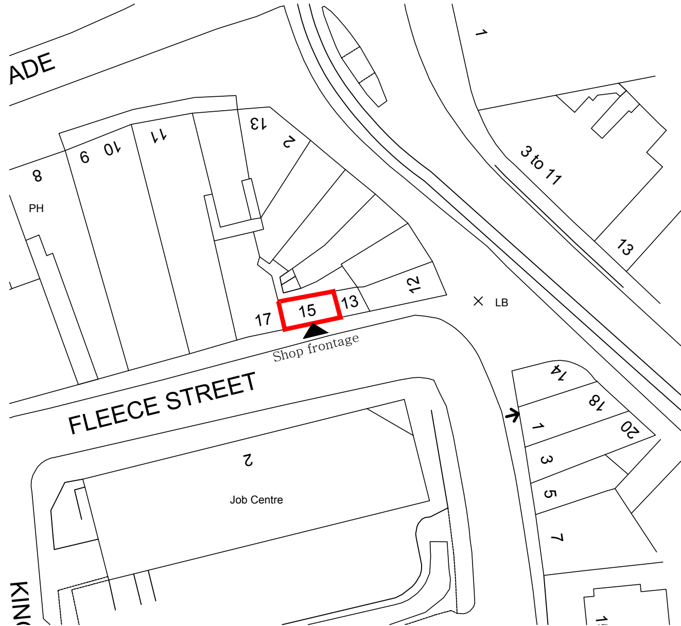
Block plan 1:500
