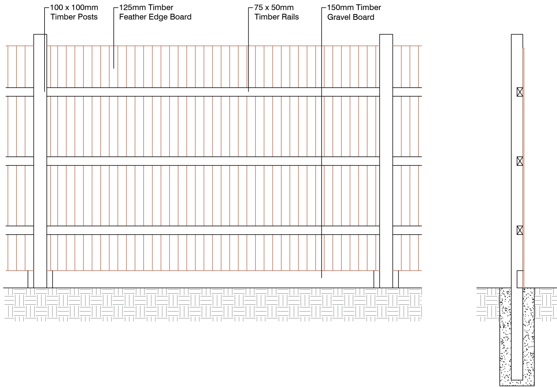
PROPOSED TIMBER FENCE DETAIL SCALE 1:20
