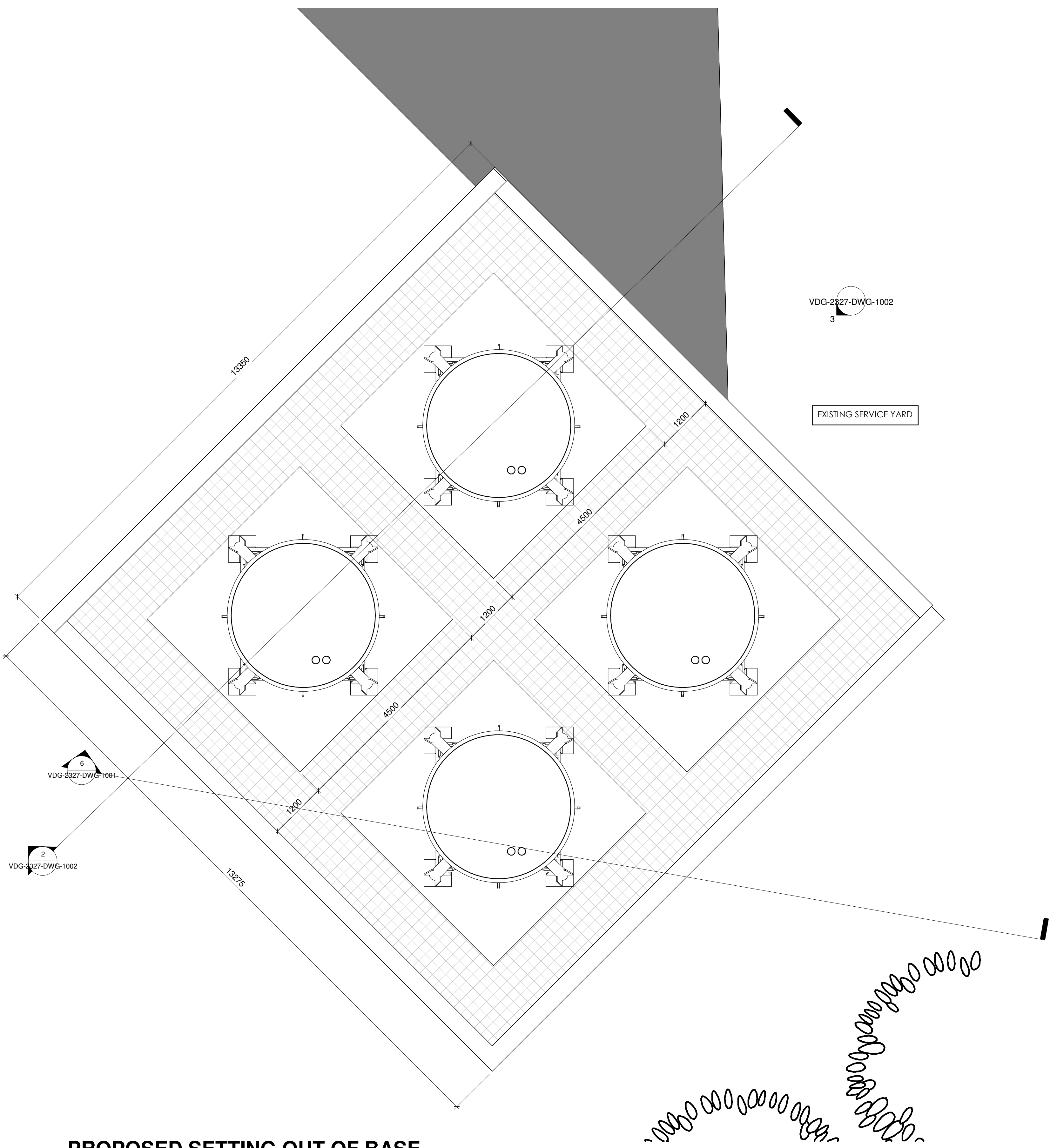
PROPOSED SETTING OUT OF BASE 1 : 50
