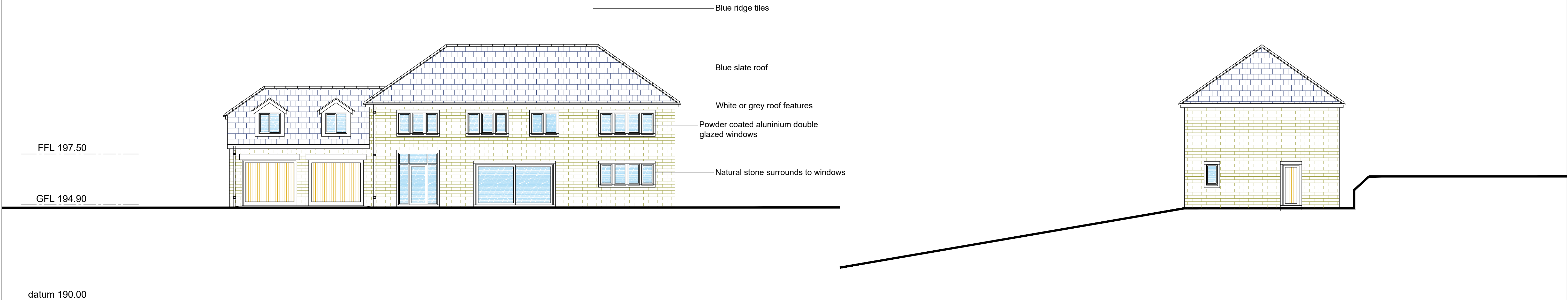
SOUTH ELEVATION
