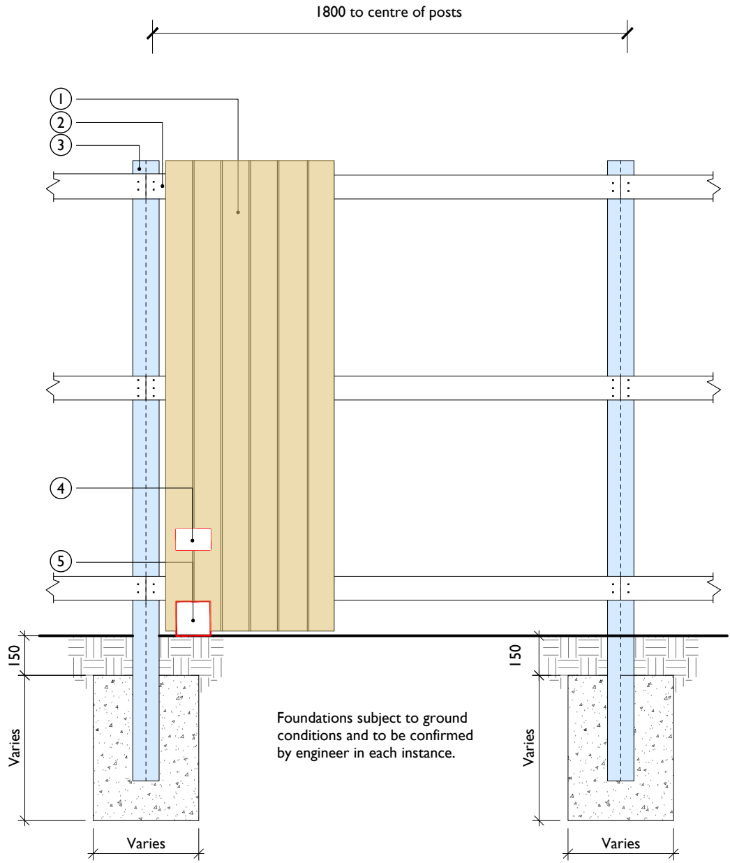
1.8m Screen fence
