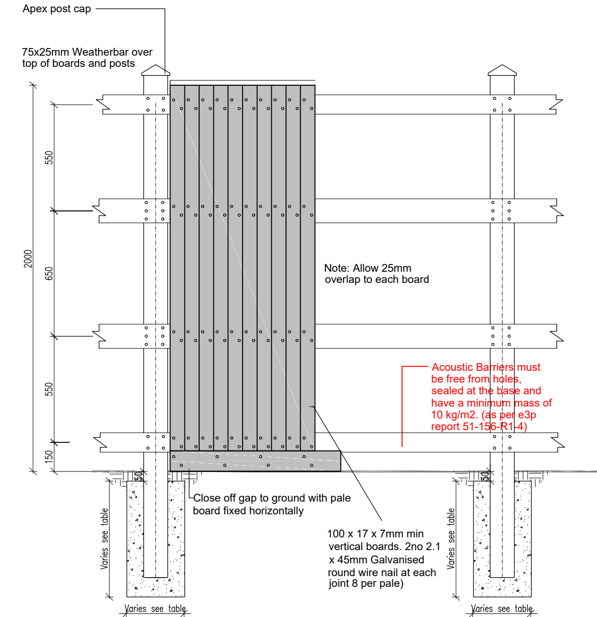
Acoustic Fence 2000-3500mm
