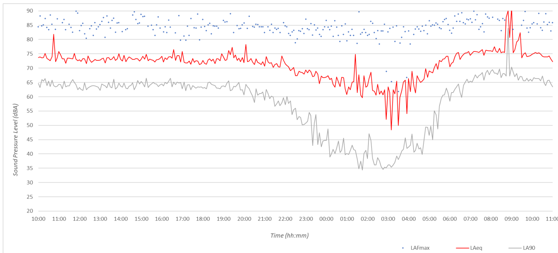
Environmental Noise Measurement M1 Time History: 4 th – 5 th June 2025
