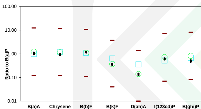
Graph 4-1: The ratio of PAH to B(a)P in soil for all available data at the site based on 5 samples (where values were >LOD to allow the calculation of a ratio).
