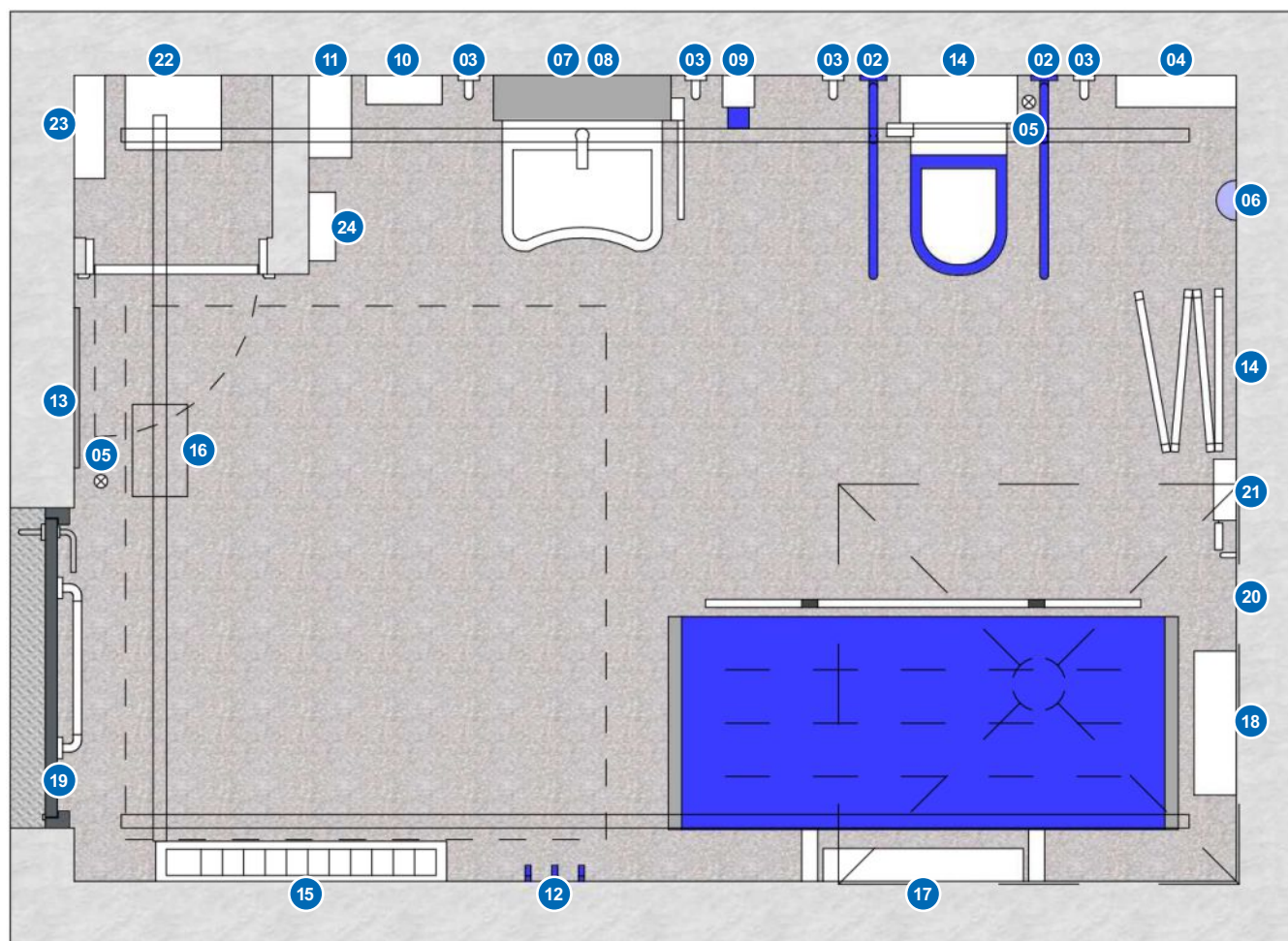
Standard internal layout of RISE CP Pod
