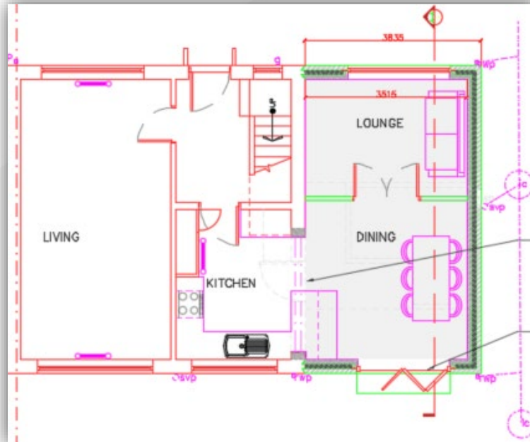
Figure 3: Proposed Ground Floor Plan, Drawing No. 24-03-01 02. (Techdlttd)
