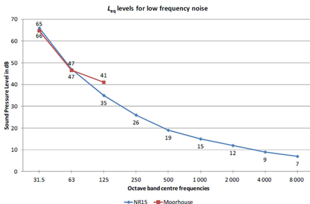
Figure 5 – Moorhouse Low Frequency Noise Rating Curve
