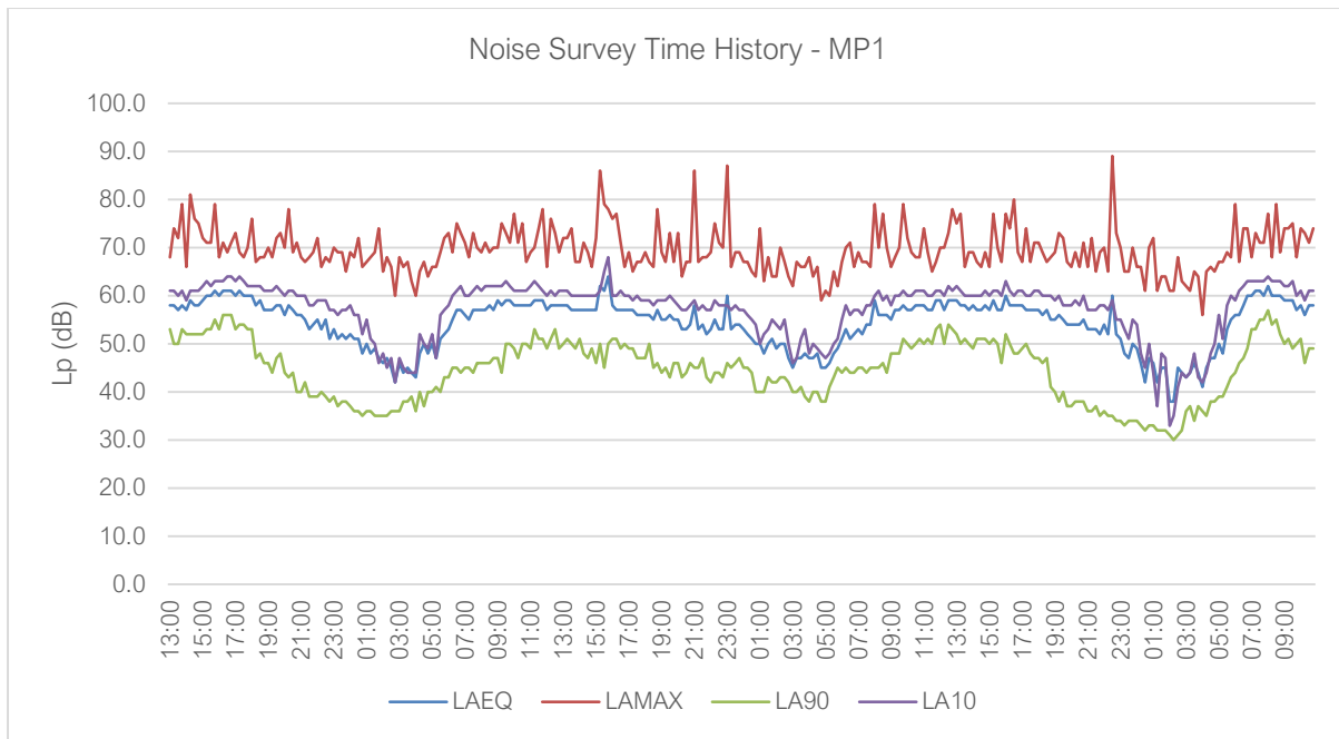
Figure 6 – Noise Survey Time History
