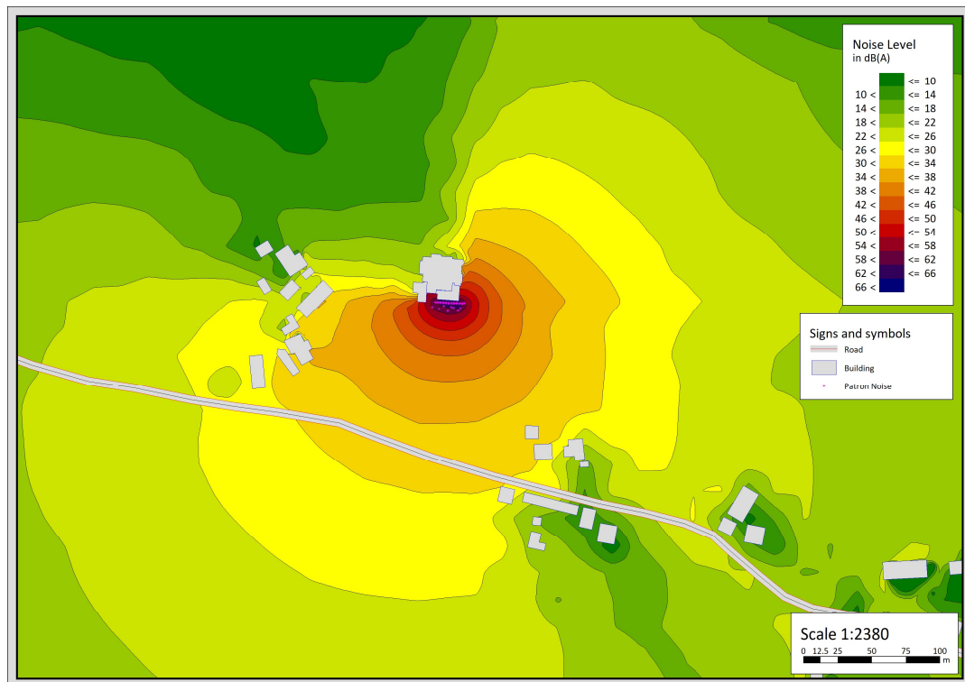
Figure 4 – Patron Noise Map – 1.5m Grid Map Height
