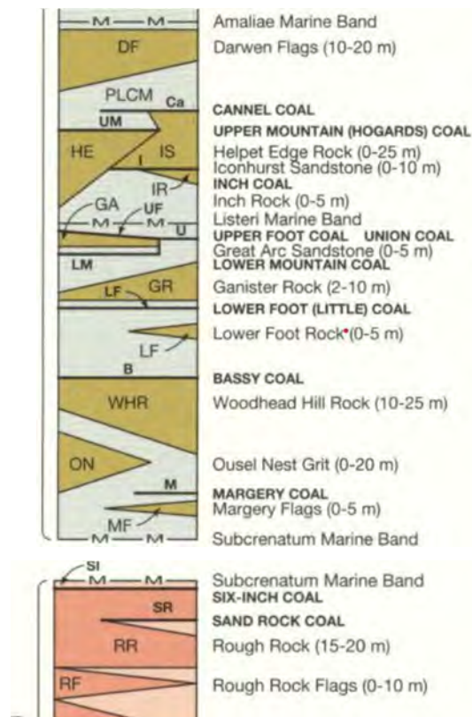
Figure 14; Extract of the BGS generalised vertical section
