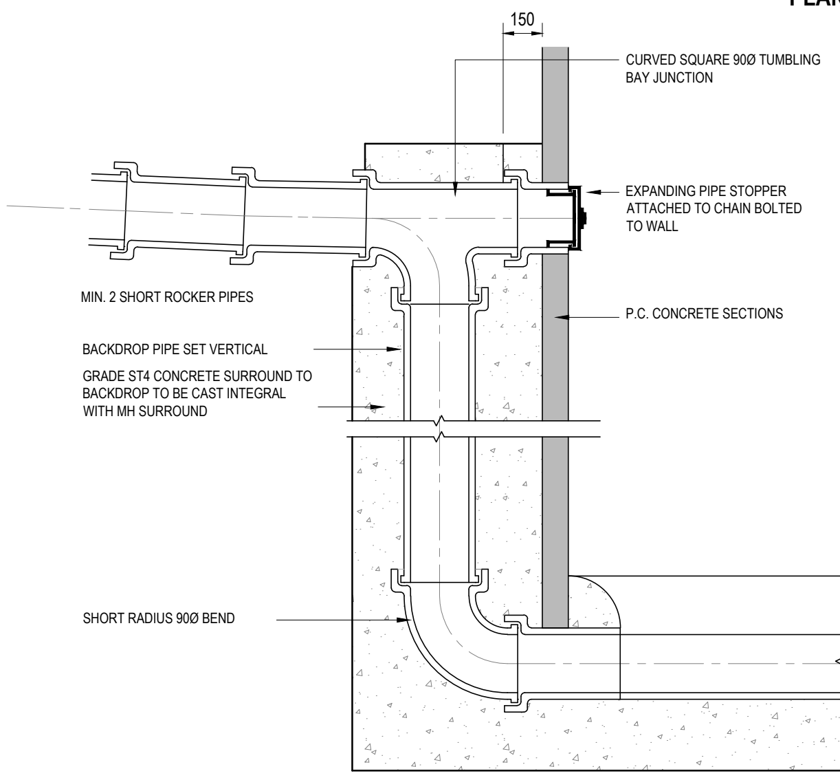
TYPICAL VERTICAL BACKDROP Scale 1:20
