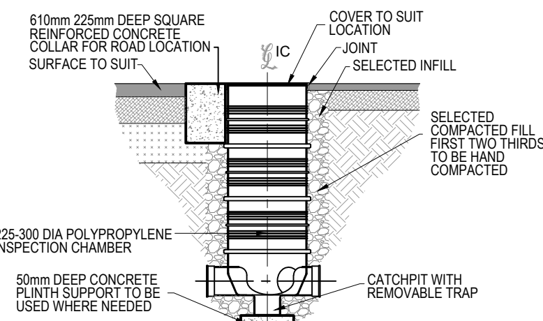
PE SHALLOW INSPECTION CHAMBER DETAIL Scale 1:20
