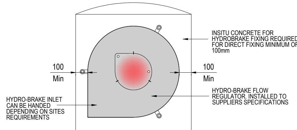
ELEVATION ON HYDRO-BRAKE DIRECT FITTING DETAIL RESTRICTION HYDRO-BRAKE DIRECT CONNECTION Scale 1:20
