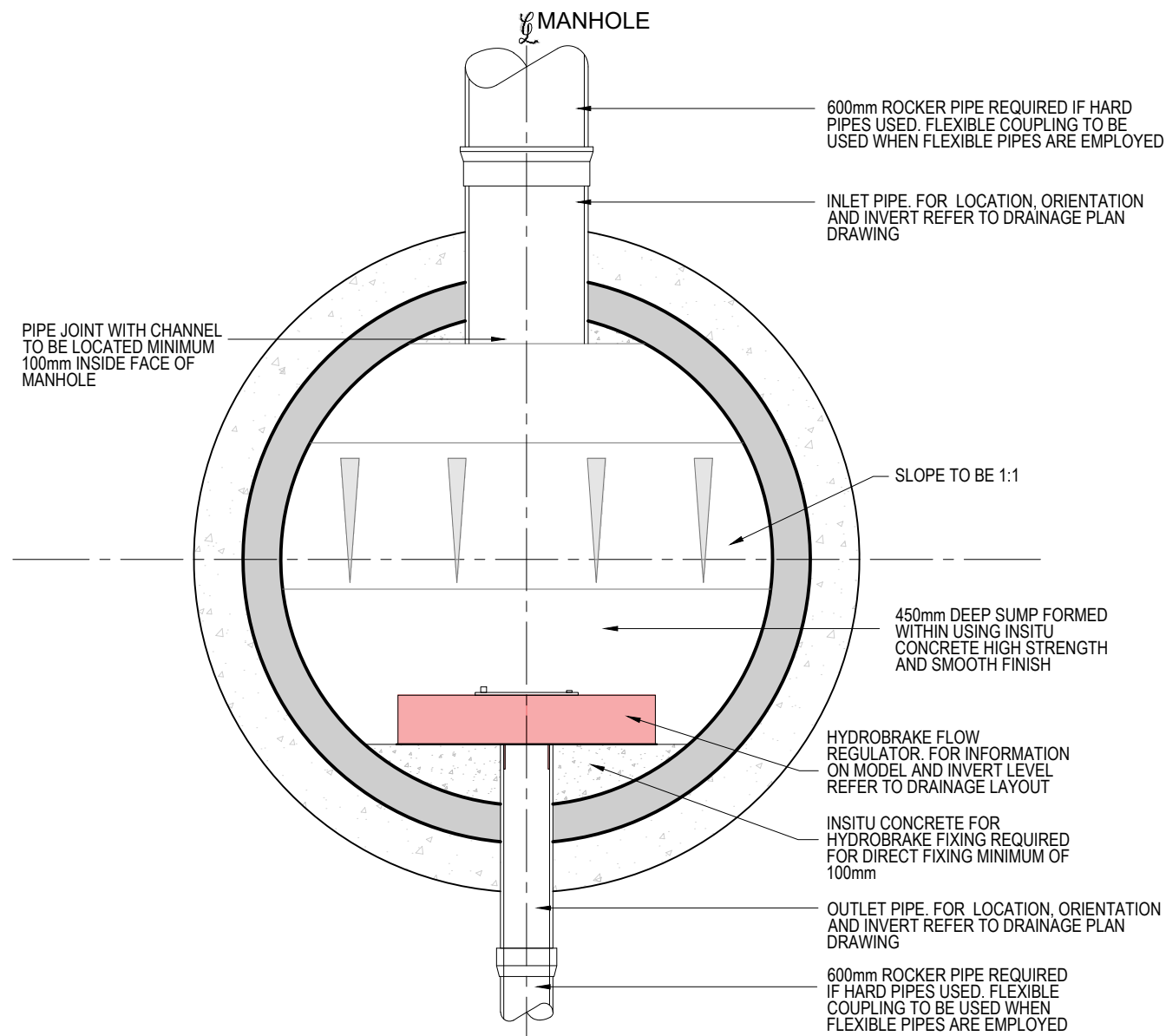
PLAN DETAIL THROUGH HYDRO-BRAKE MANHOLE RESTRICTION HYDRO-BRAKE DIRECT CONNECTION Scale 1:20
