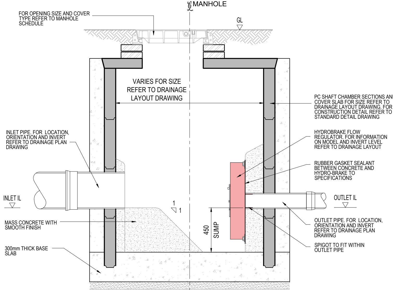
SECTIONAL DETAIL THROUGH HYDRO-BRAKE MANHOLE RESTRICTION HYDRO-BRAKE DIRECT CONNECTION Scale 1:20
