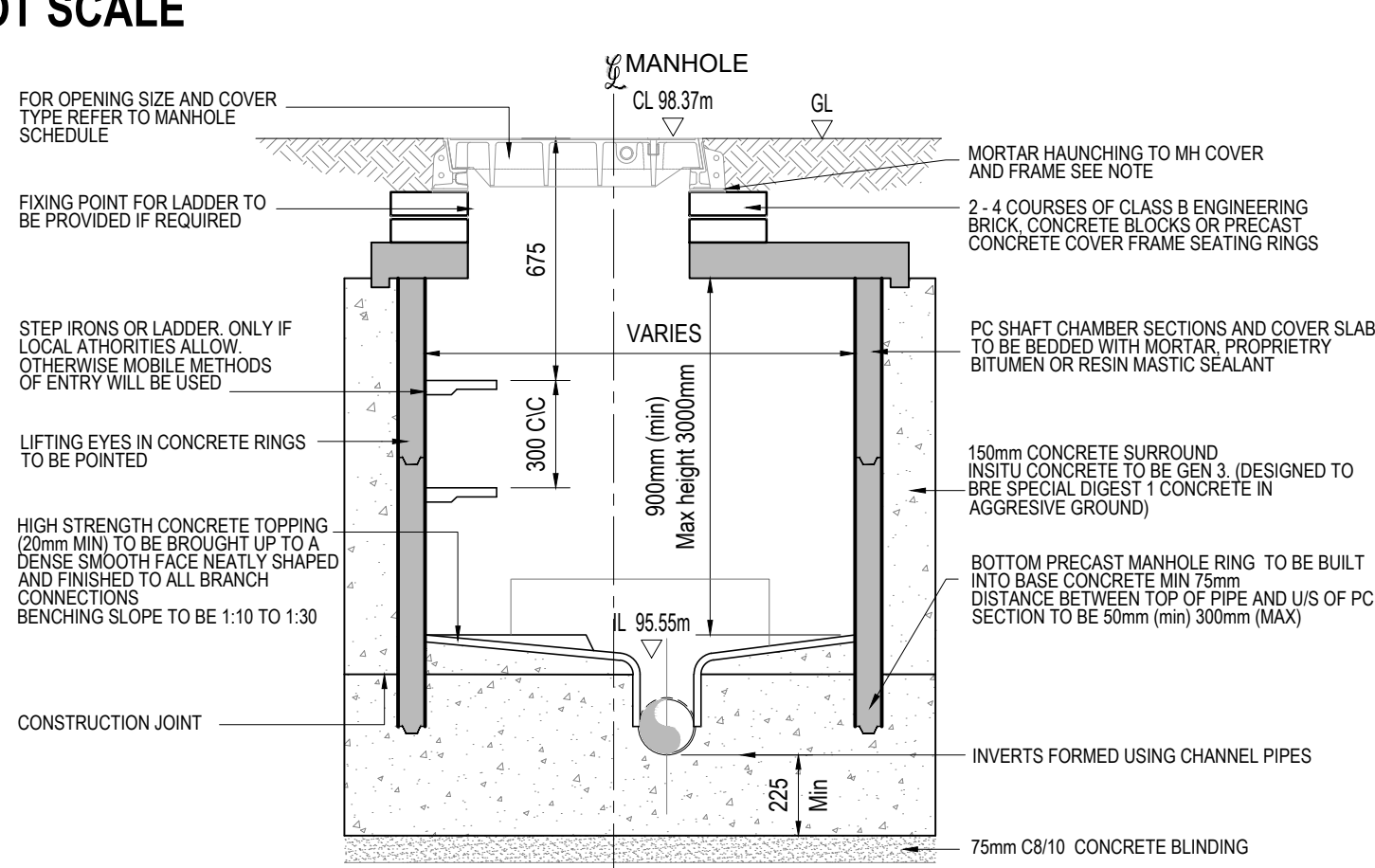
PROPOSED PC CONCRETE MANHOLE ON EXISTING SEWER SECTION DETAIL Scale 1:20
