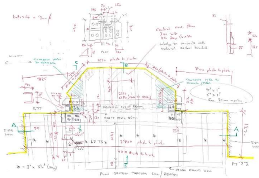
Detailed survey by architect of existing oriel window support structure
