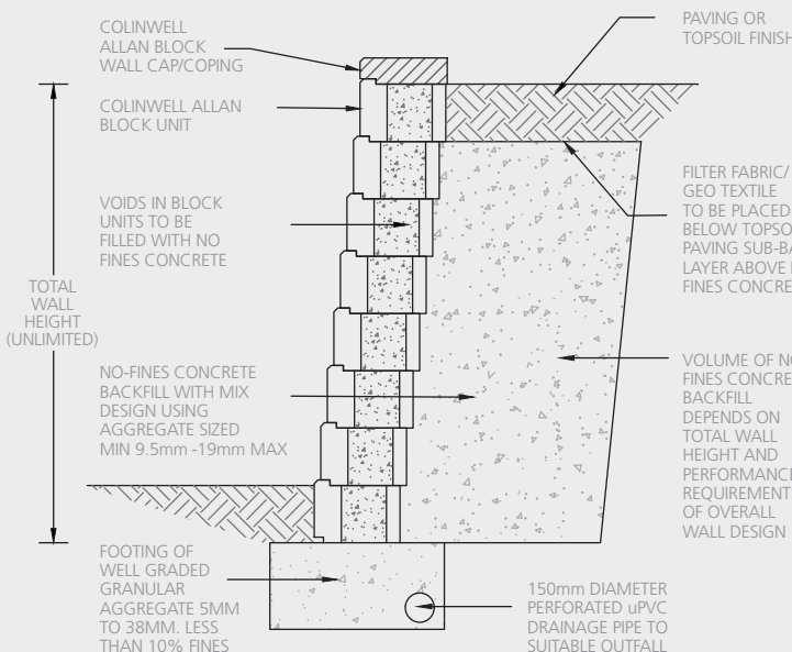
Illustration 2 Depth of No-Fines Concrete backfill is determined by overall wall height and potential loading on finished wall.
