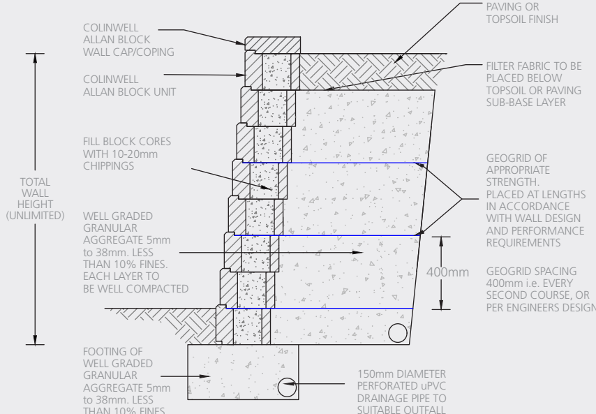
Illustration 1 Geogrid Lengths/Tails are determined by overall wall height and potential loading on finished wall.
