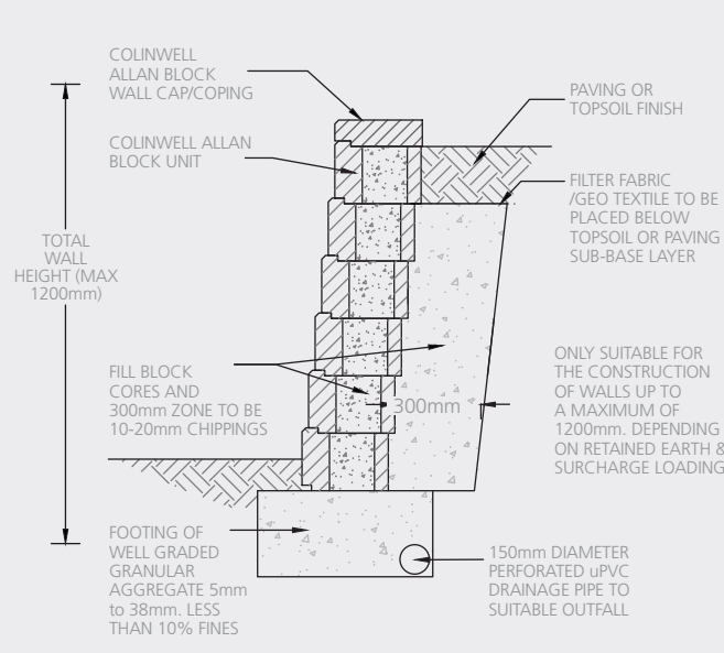
Illustration 3 Only suitable for the construction of walls up to a maximum of 1200mm as illustrated above
