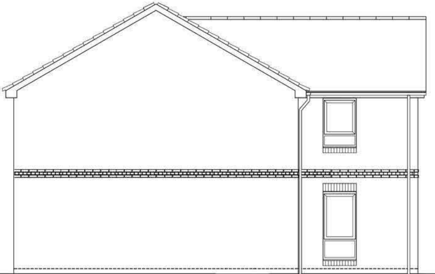
SIDE (LEFT) ELEVATION DETACHED EMG43 (4B7P)
