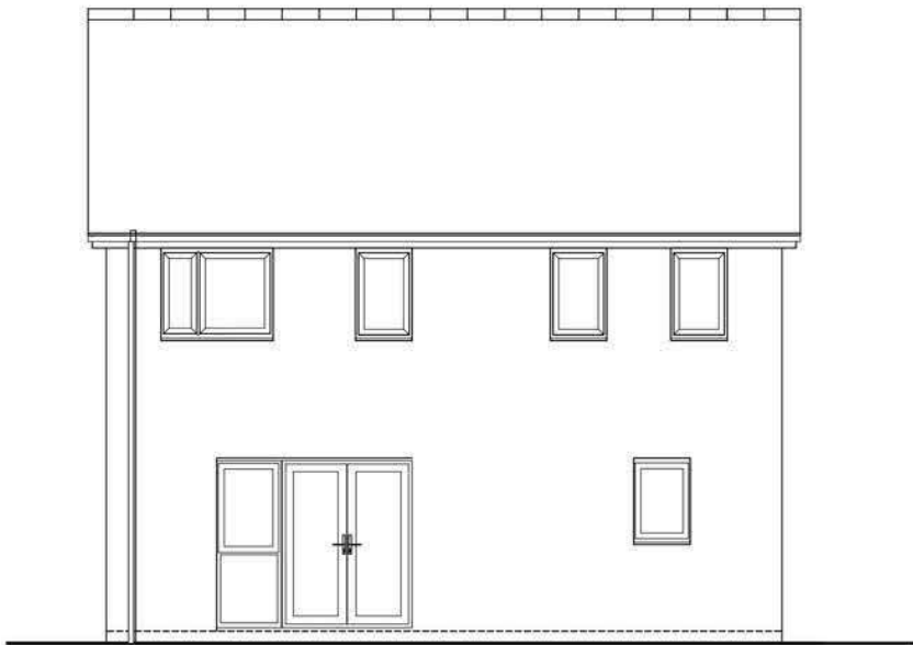
REAR ELEVATION DETACHED EMG3 I (3B5P)
