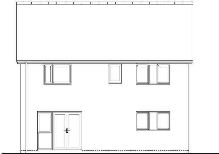
REAR ELEVATION DETACHED EMA46 (4B7P)
