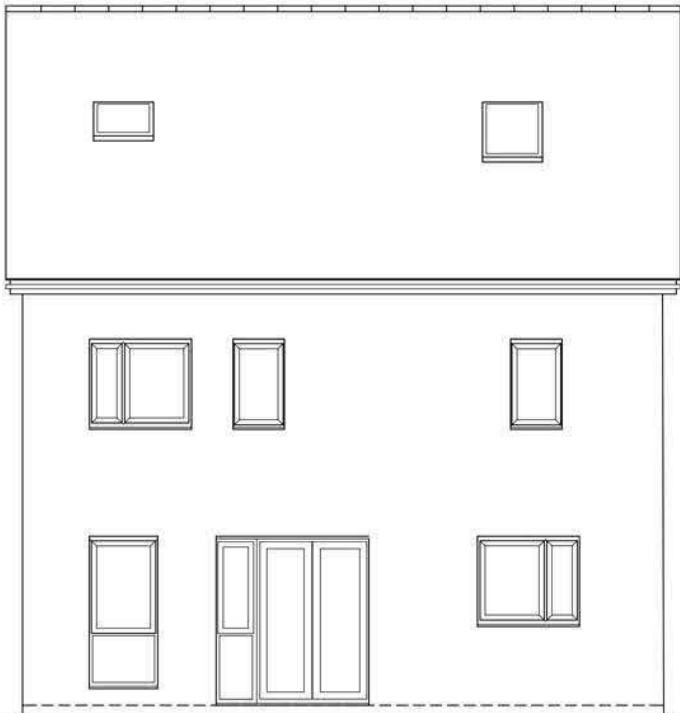
REAR ELEVATION DETACHED EMB5 I (5B7P)
