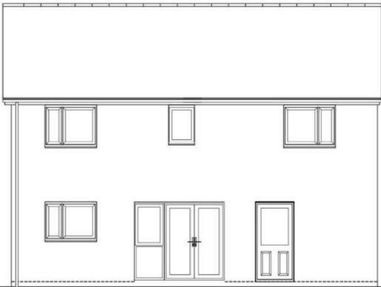
REAR ELEVATION DETACHED EMG43 (4B7P)
