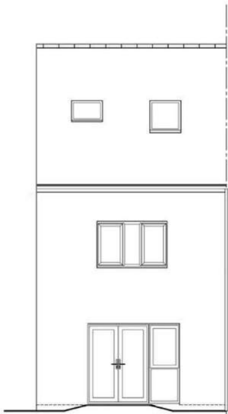
REAR ELEVATION END/SEMI DETACHED EMB3 I (3B5P)
