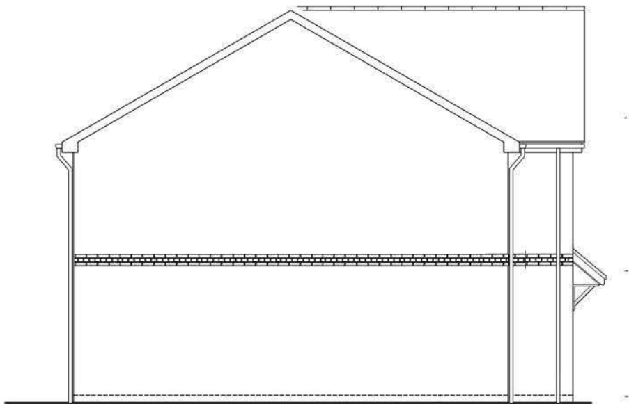
SIDE ELEVATION DETACHED EMG3 I (3B5P)
