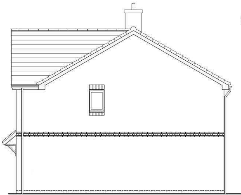
SIDE ELEVATION DETACHED EMG3 I (3B5P)
