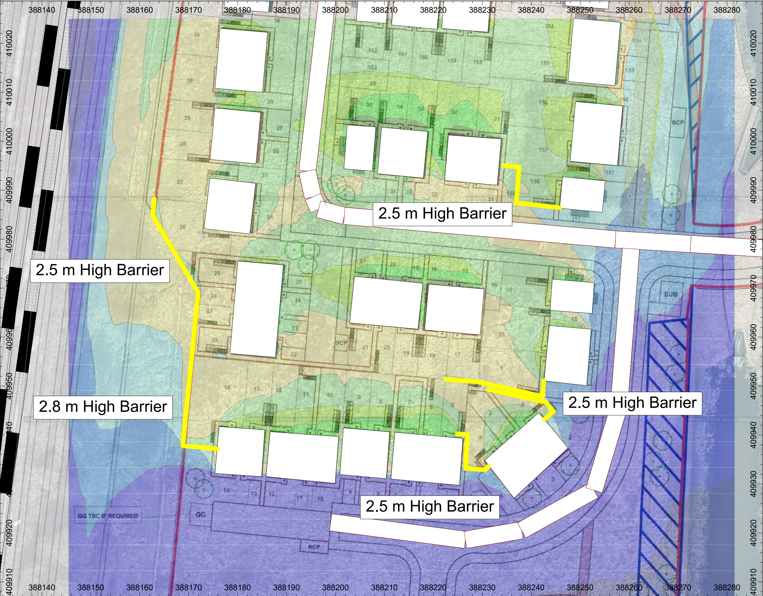
Figure 7 - Daytime Grid Noise Map with Mitigation - Calculation at 1.5 m above ground level
