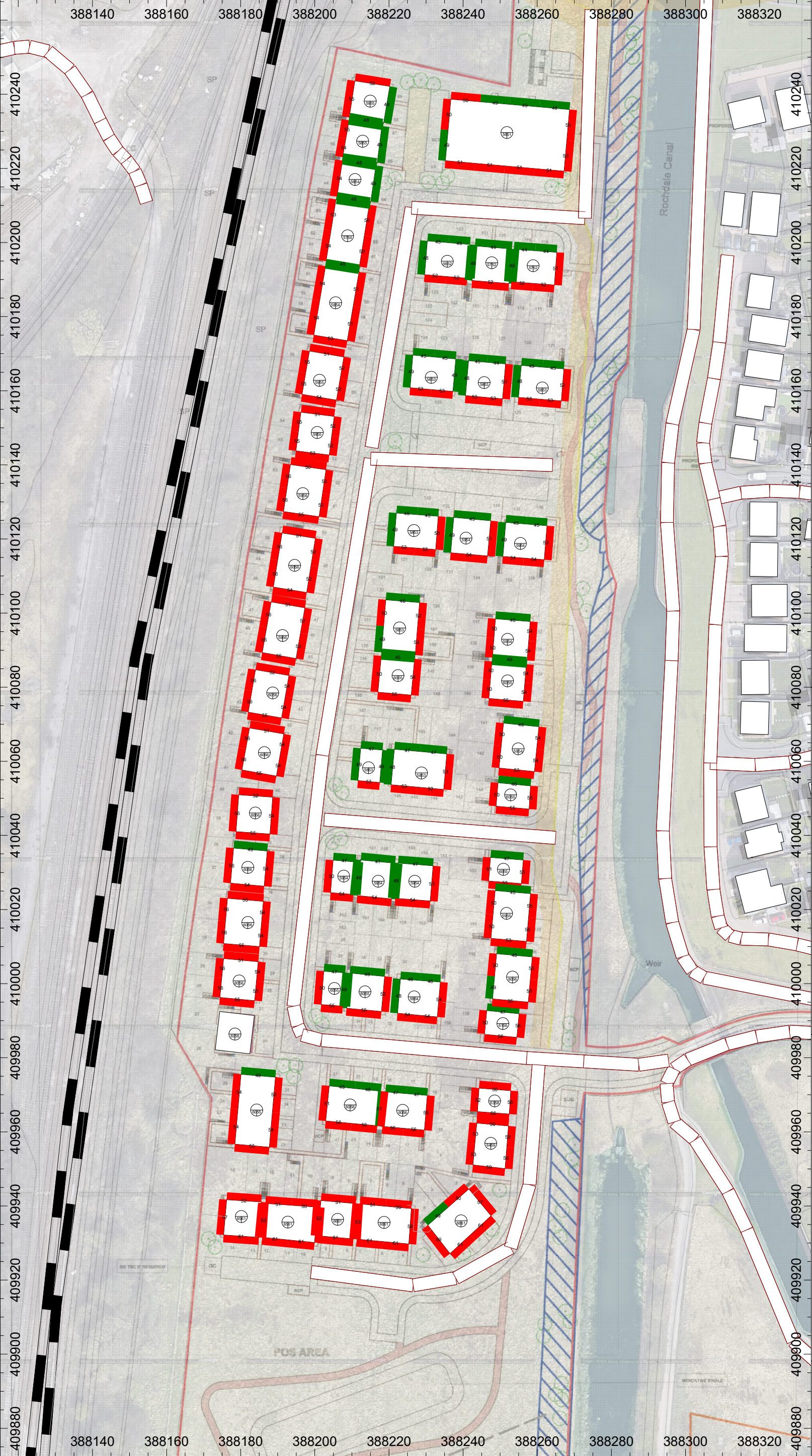
Figure 6 - Night-time Grid Noise Map (Part 0) - Calculation at 4.5 m above ground level
