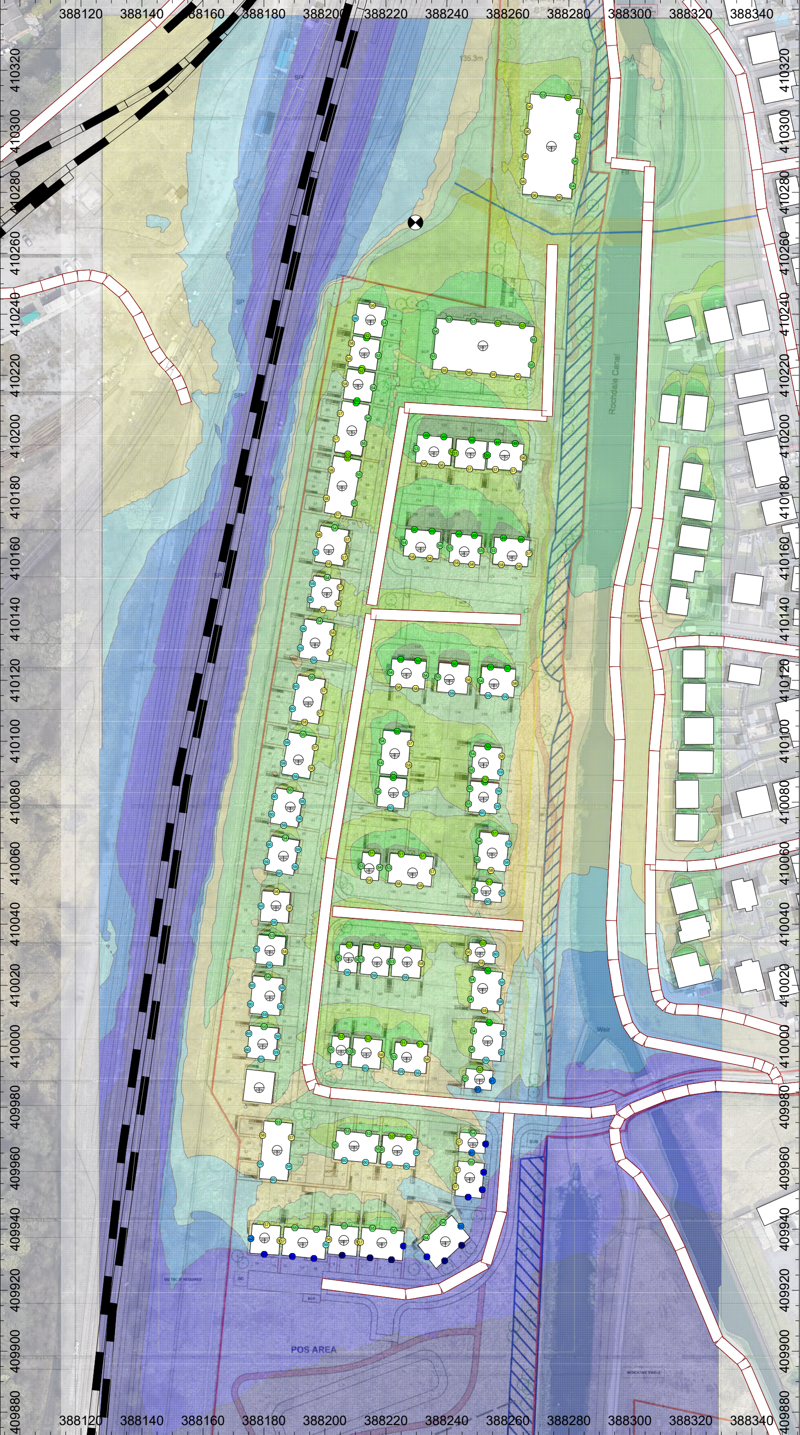
Figure 3 - Daytime Grid Noise Map (BS 8233) - Calculation at 1.5 m above ground level
