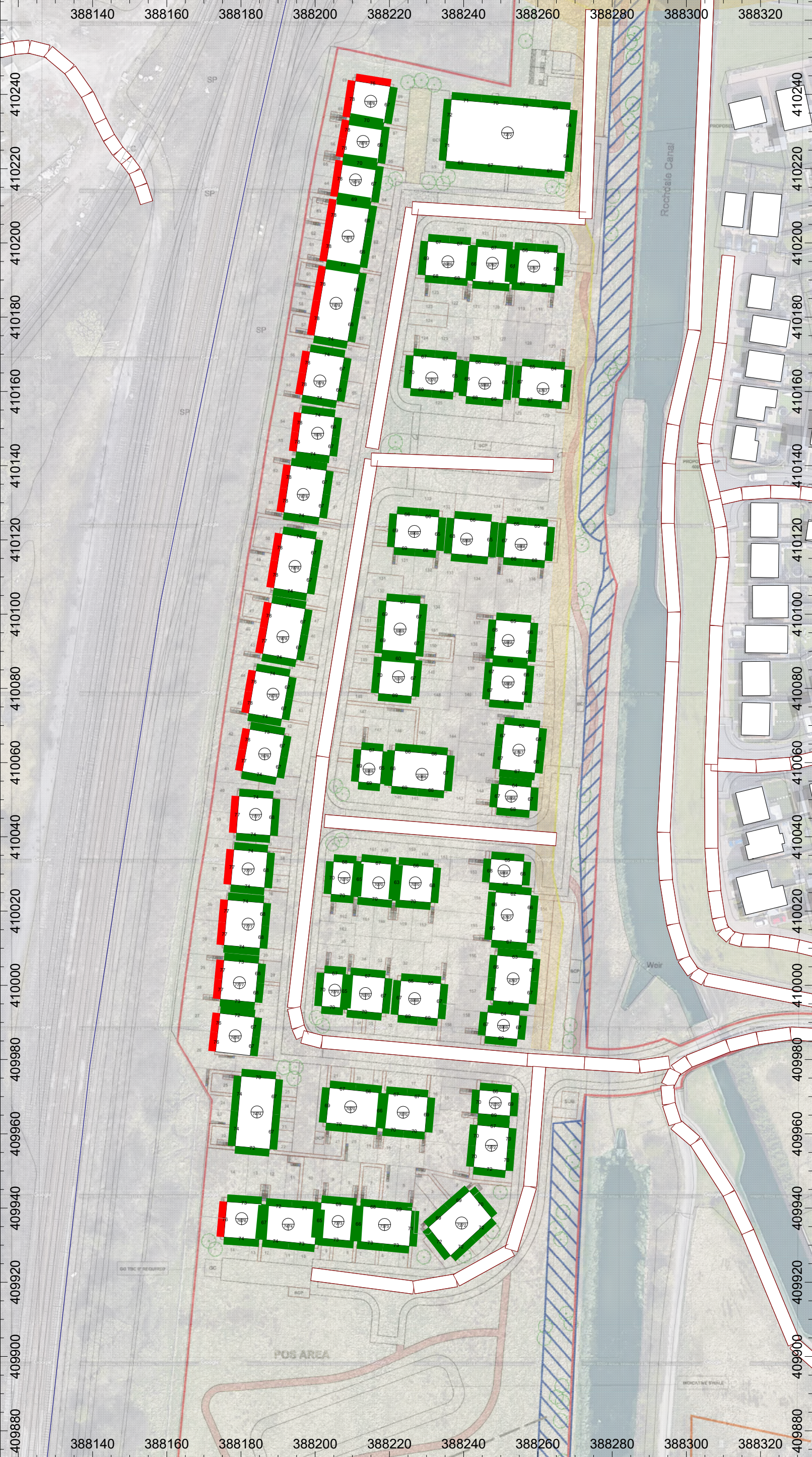
Figure 5 - 10th Highest Maximum Night-time Grid Noise Map (BS 8233) - Calculation at 4.5 m above ground level
