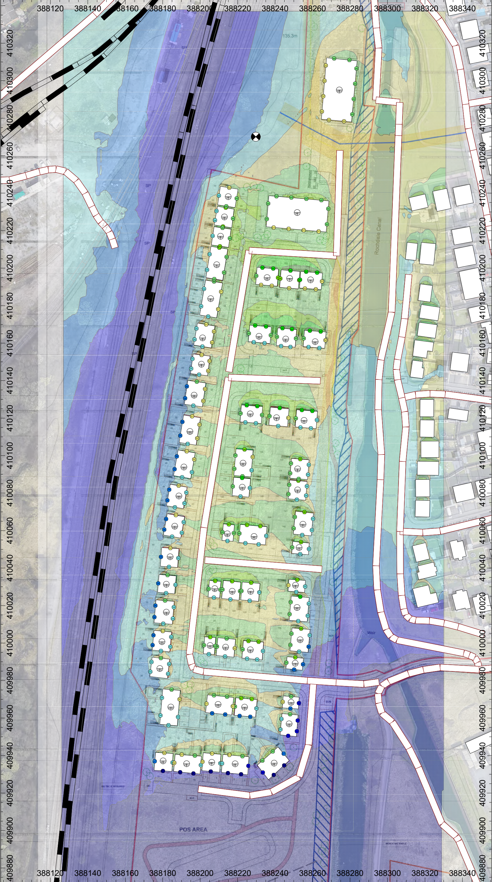
Figure 4 - Night-time Grid Noise Map (BS 8233) - Calculation at 4.5 m above ground level
