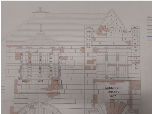
Drawing annotated with the masonry references
