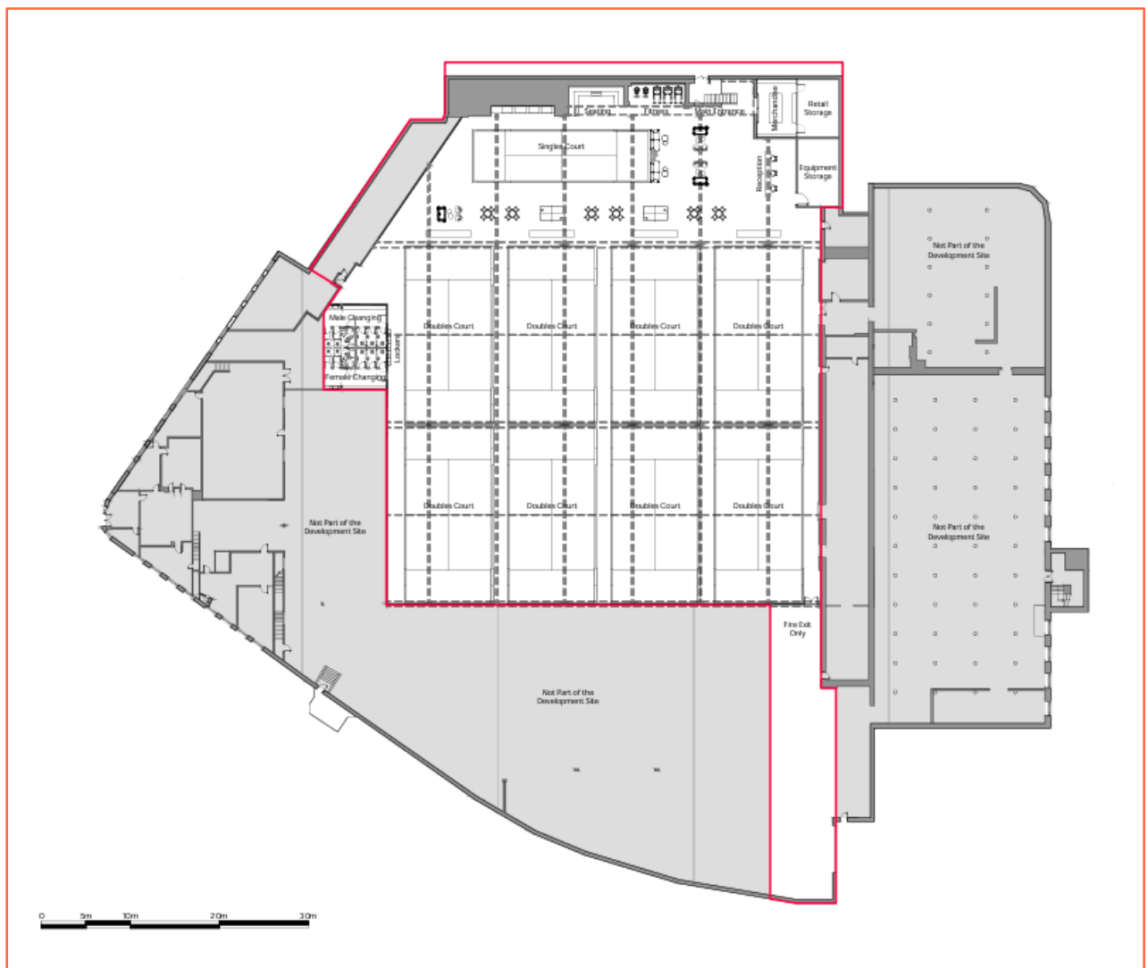
Figure 3: Proposed ground floor plan (Source: NC Studio)
