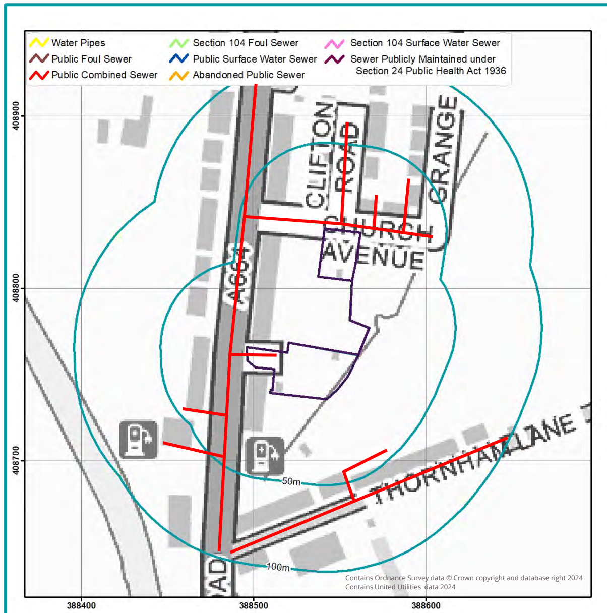
Figure 7. Sewer features map (OS & United Utilities, 2024)
