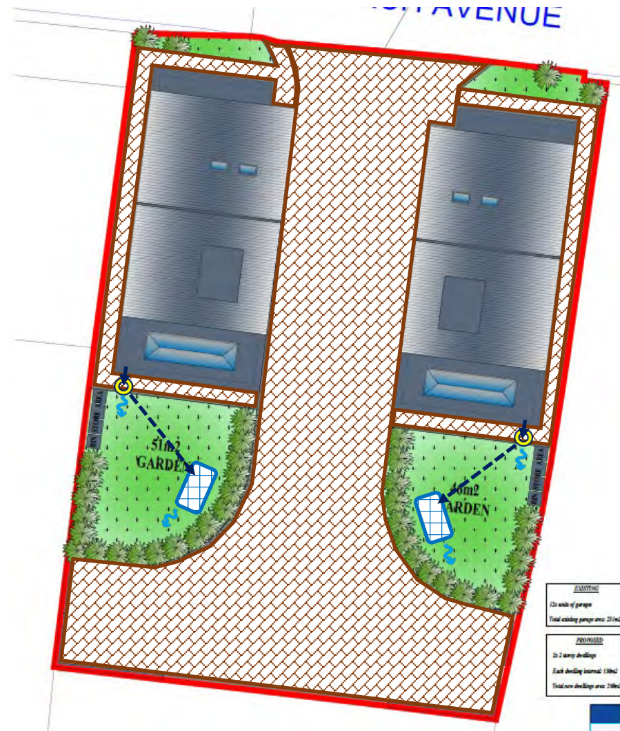
Figure 1. Proposed SuDS scheme layout– Site 1 (north)
