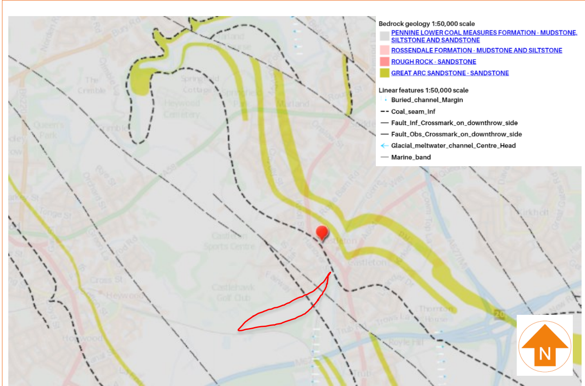
Figure 3.2 SNAPSHOT OF BEDROCK GEOLOGY AND FAULTING
