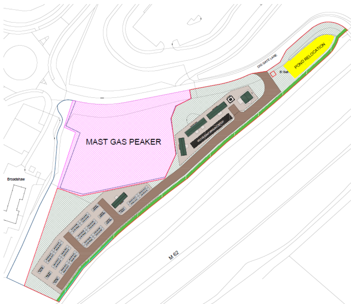
Figure 3: Proposed Site Layout Plan
