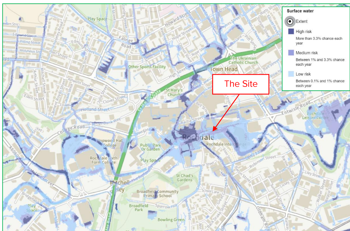
Figure 11 - Environment Agency Surface Water Flood Map
