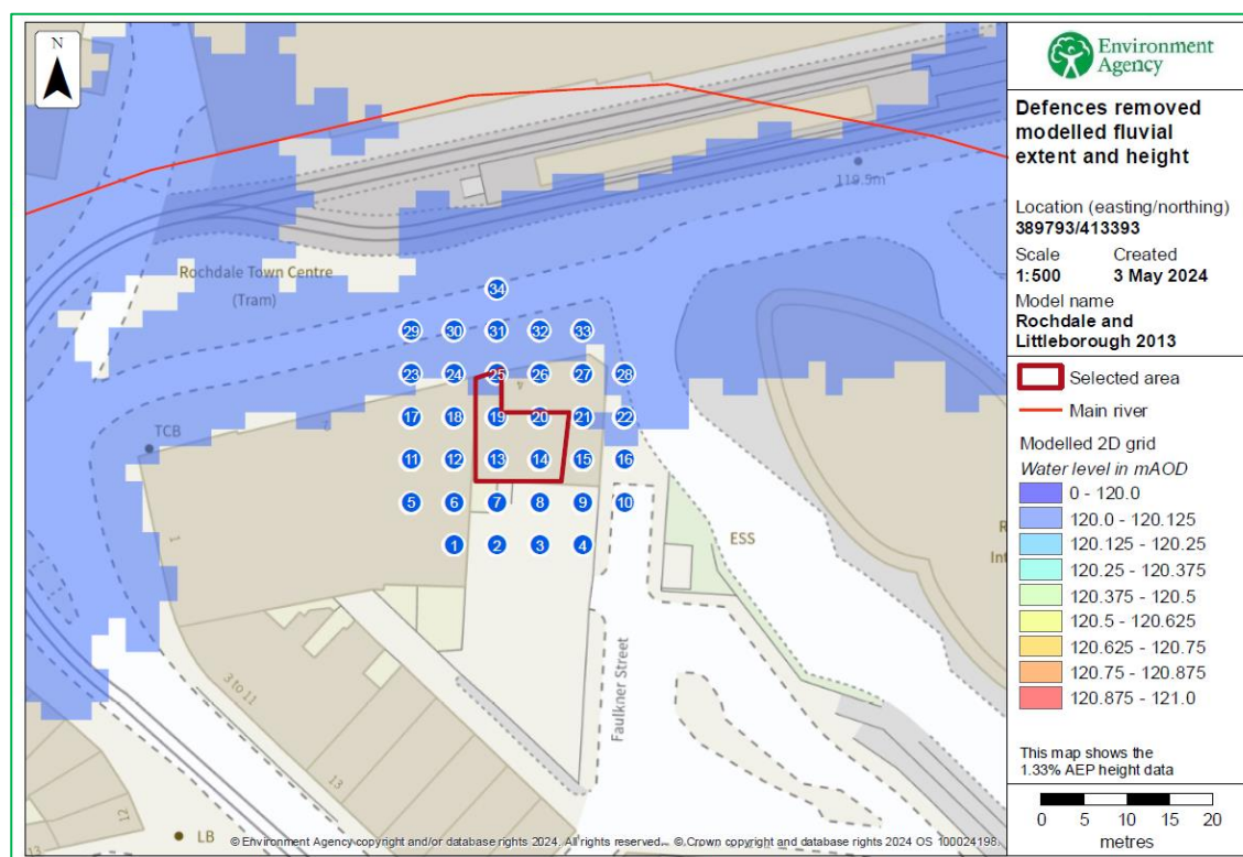
Figure 10 - Environment Agency Modelled Nodes Location Map Undefended 1 in 75 Year Event
