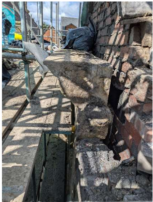
Gable dismantled down to the window head detail and temporary support provided
