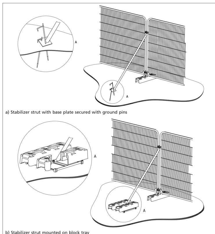
FIGURE 5: FURTHER SPECIFICATION OF TREE PROTECTION FENCING
