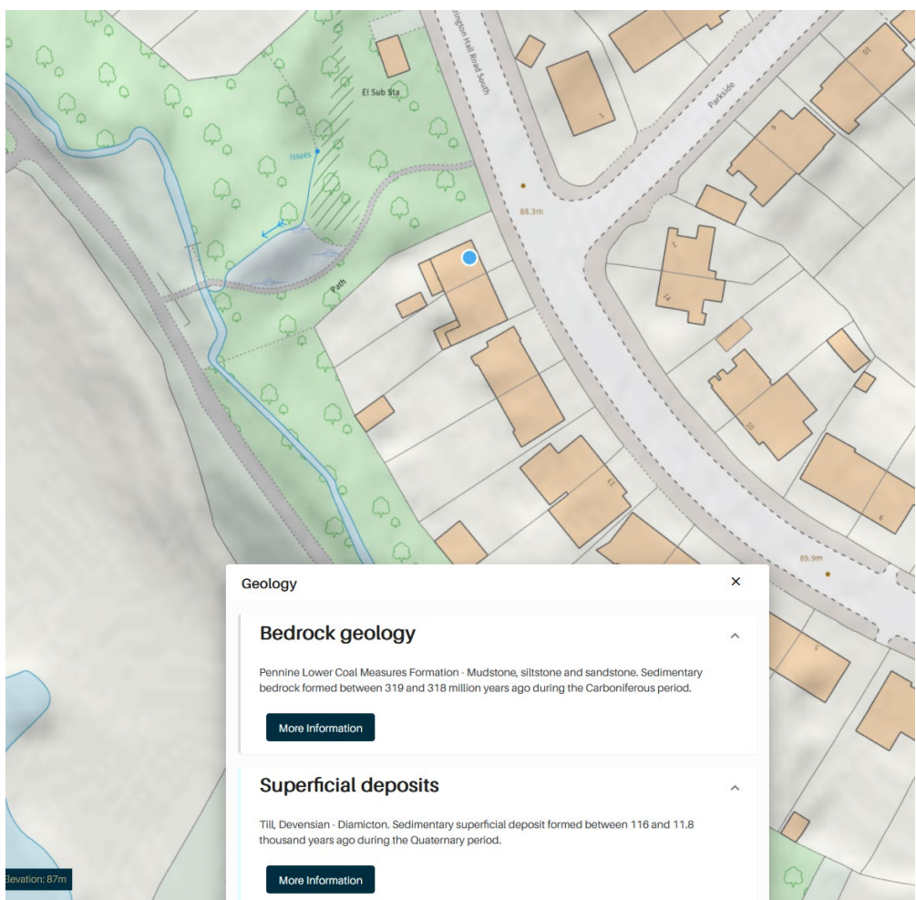
FIGURE 3: BGS GEOLOGY VIEW SHOWING BEDROCK FORMATION AND SUPERFICIAL DEPOSITS
