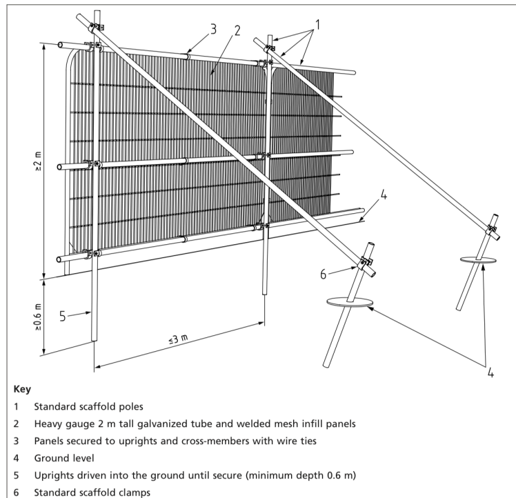
FIGURE 4: SPECIFICATION FOR TREE PROTECTION FENCING FROM BS5837
