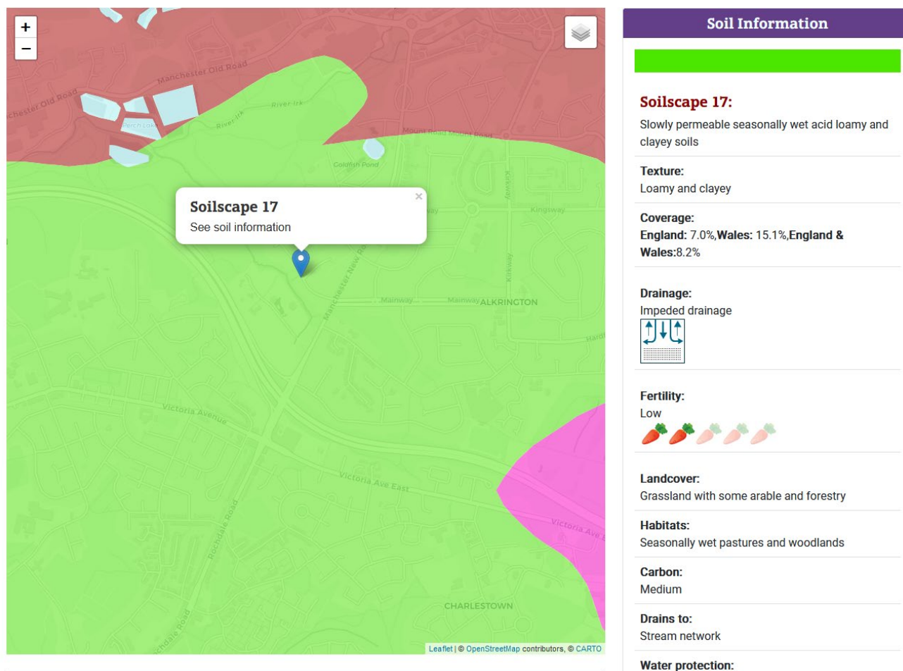
FIGURE 2: SOILSCAPES APP SHOWING SOIL TYPES
