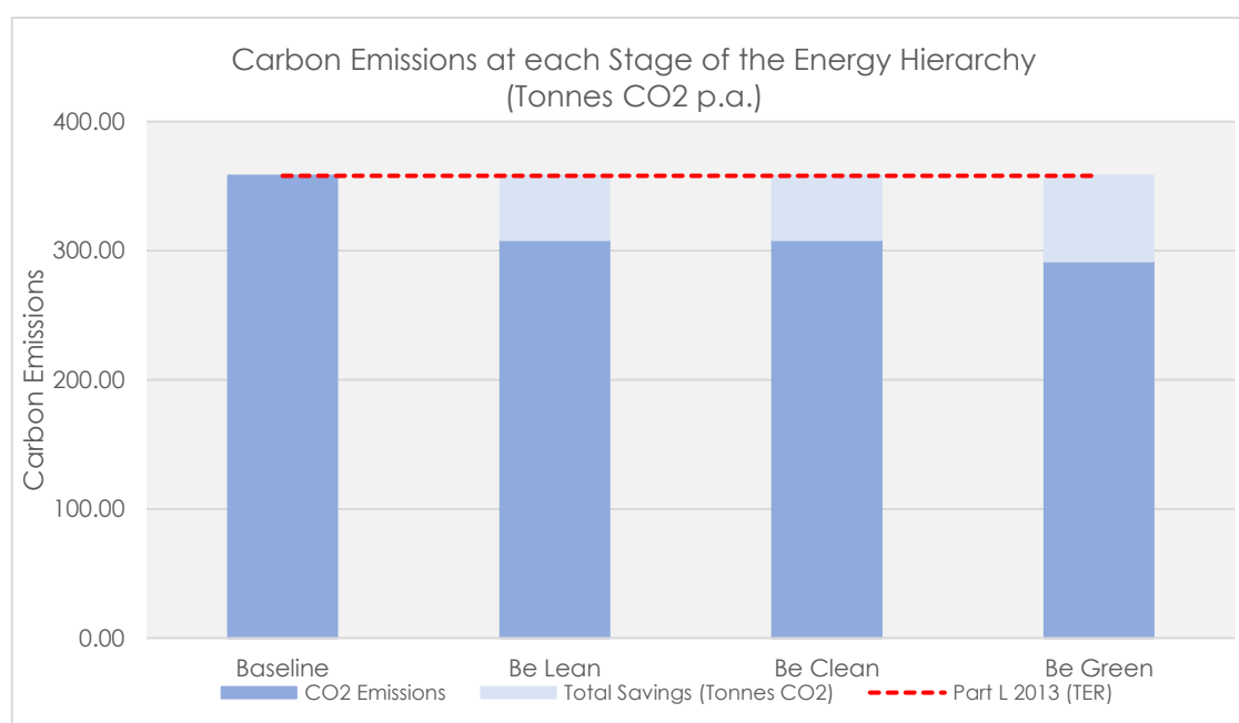
Figure 8.1: Proposed Development CO 2 Reduction Hierarchy
