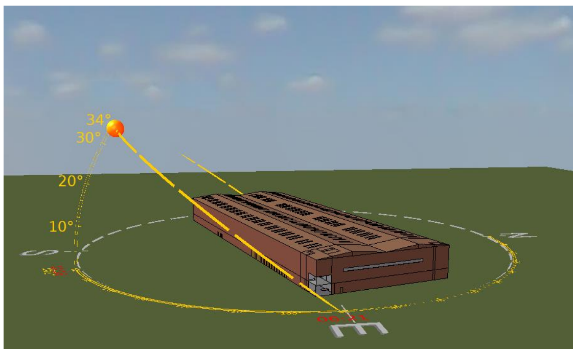
Figure 1.1: Proposed Development Thermal Model (Unit J1 only) in IES VE
