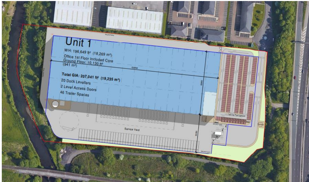
Figure 4.1 Site Layout
