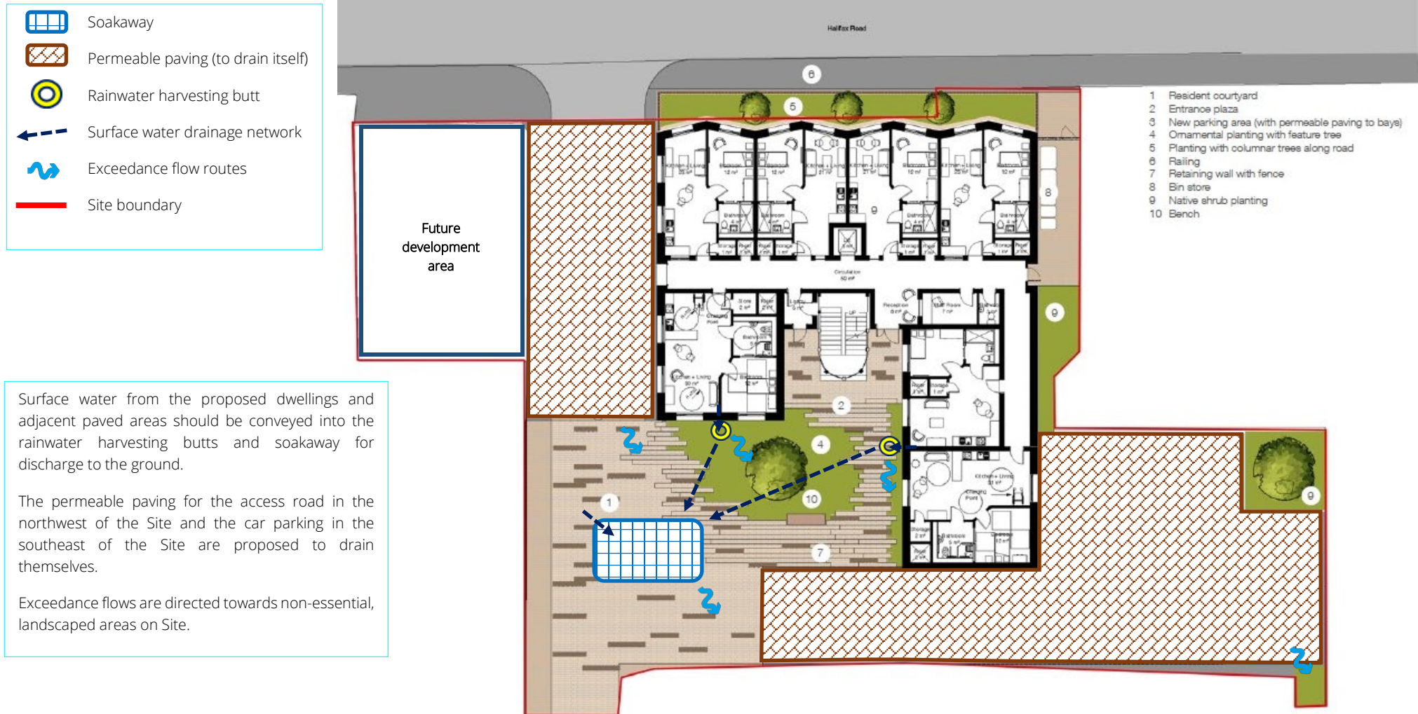
Figure 1. Proposed SuDS scheme
