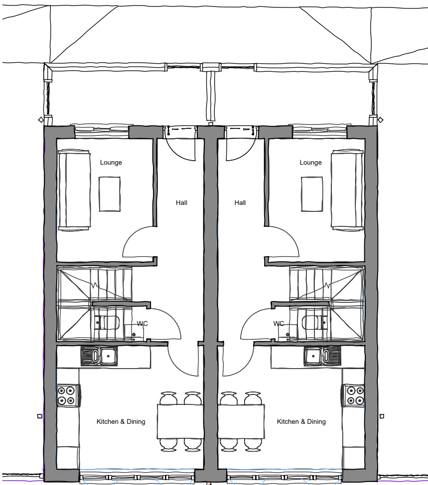
00-0F-UNIT TYPE PLAN 1:100 @ A1
