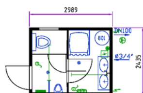
Sanitary cabin 10'
