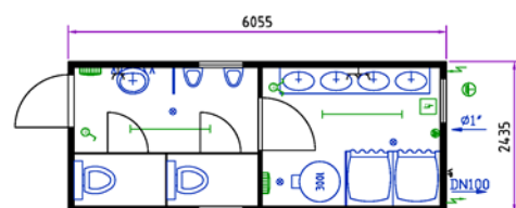
Sanitary cabin 20'
