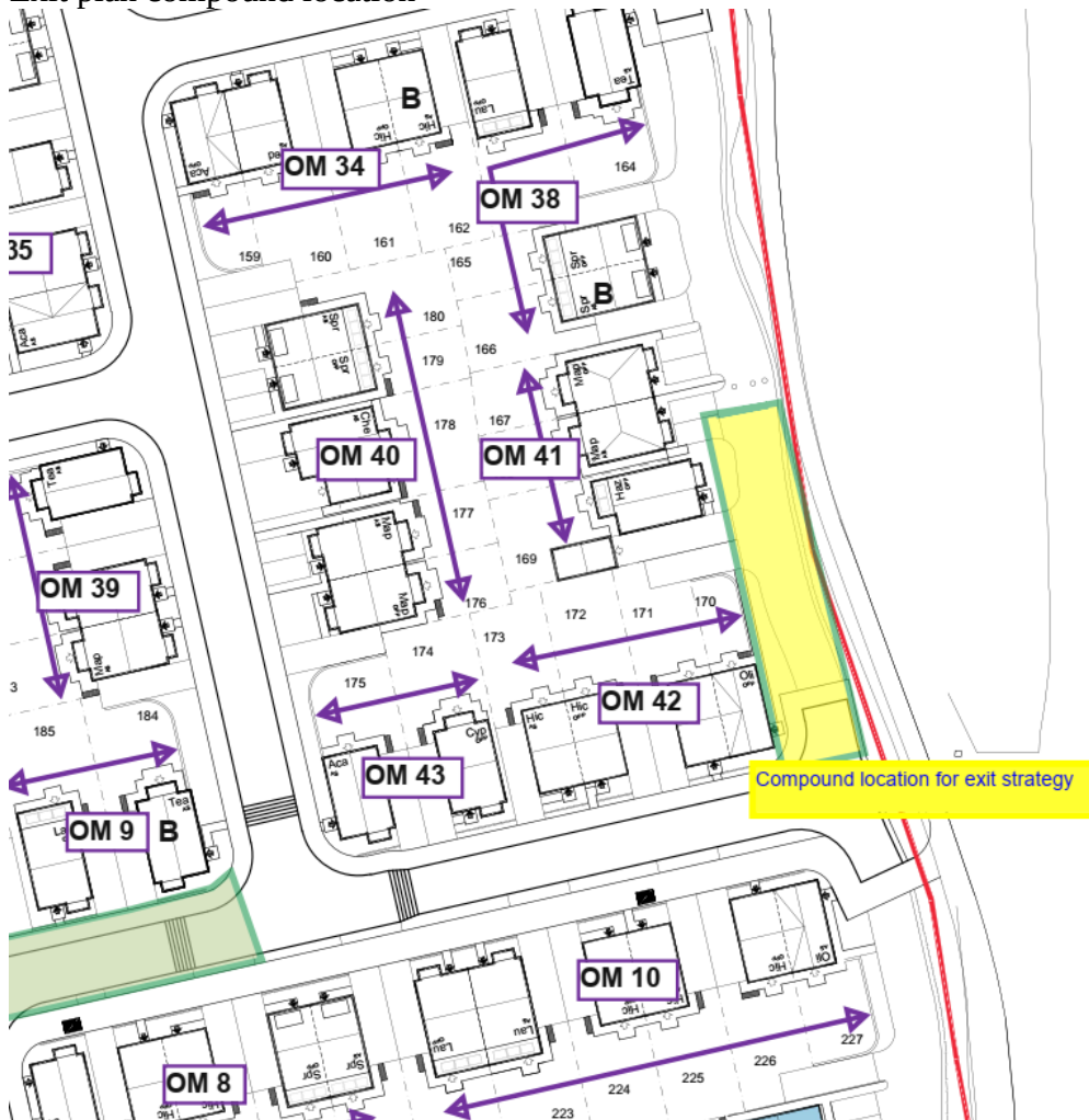
Exit plan compound location
