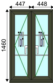
1 - 895w x 1490h, 30mm Cill Viewed Outside Style No: 18
