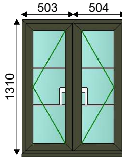
1 - 1007w x 1310h (Basic Frame Size) 30 mm Cill
