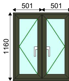
1 - 1002w x 1160h (Basic Frame Size) 1 - 1002w x 1190h, 30mm Cill
