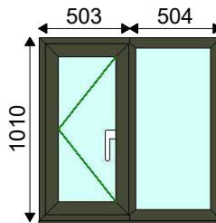
1 - 1007w x 1010h (Basic Frame Size) 1 - 1007w x 1040h, 30mm Cill Viewed Outside Style No: 16
