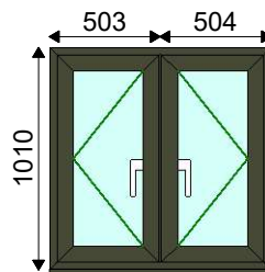
1 - 1007w x 1010h (Basic Frame Size) 1 - 1007w x 1040h, 30mm Cill Viewed Outside Style No: 18
