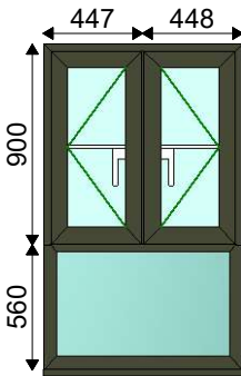
1 - 895w x 1490h, 30mm Cill Viewed Outside Style No: (Custom)
