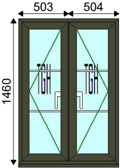
1 - 1007w x 1490h, 30mm Cill Viewed Outside Style No: 18
