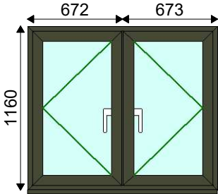
1 - 1345w x 1160h (Basic Frame Size) 1 - 1345w x 1190h, 30mm Cill
